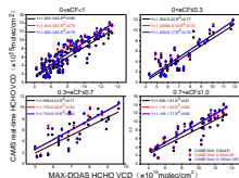
Figure S4: Correlation between HCHO VCDs retrieved from the MAX-DOAS measurements and those obtained from the CAMS model for 0 \leq cCF \leq 1 (a), 0 \leq cCF \leq 0.3 (b), 0.3 \leq cCF \leq 0.7 (c), and 0.7 \leq cCF \leq 1.0 (d) at 14:00 LT from October to December 2014.
