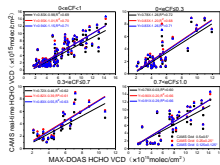
Figure S3: Correlation between HCHO VCDs retrieved from the MAX-DOAS measurements and those obtained from the CAMS model data for 0 \leq cCF \leq 1 (a), 0 \leq cCF \leq 0.3 (b), 0.3 \leq cCF \leq 0.7 (c), and 0.7 \leq cCF \leq 1.0 (d) at 8:00 LT from October to December 2014.
