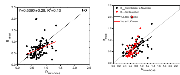
Scatter plots and linear regression of R_{max} against R_{MAX-DOAS} (see the text) from October to December 2014 (a) and from October to November and for December due to the changing of temperature (b). There are not significant differences between the two periods.
