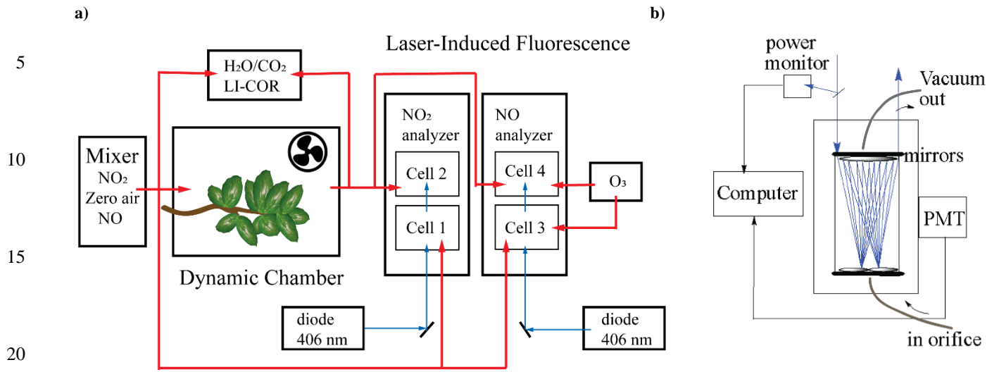
Figure 2: Schematic of the experimental dynamic chamber (a) and laser-induced fluorescence detection (b) setups.
