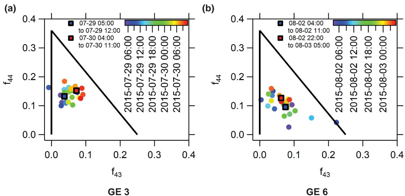
Figure 9. Scatter plot of the organic aerosol fraction measured at m/z 43 versus that measured at m/z 44 during GE 3 (a) and GE 6 (b) near Eureka. Also shown are the average values corresponding to the first seven and final seven hours of the growth event.
