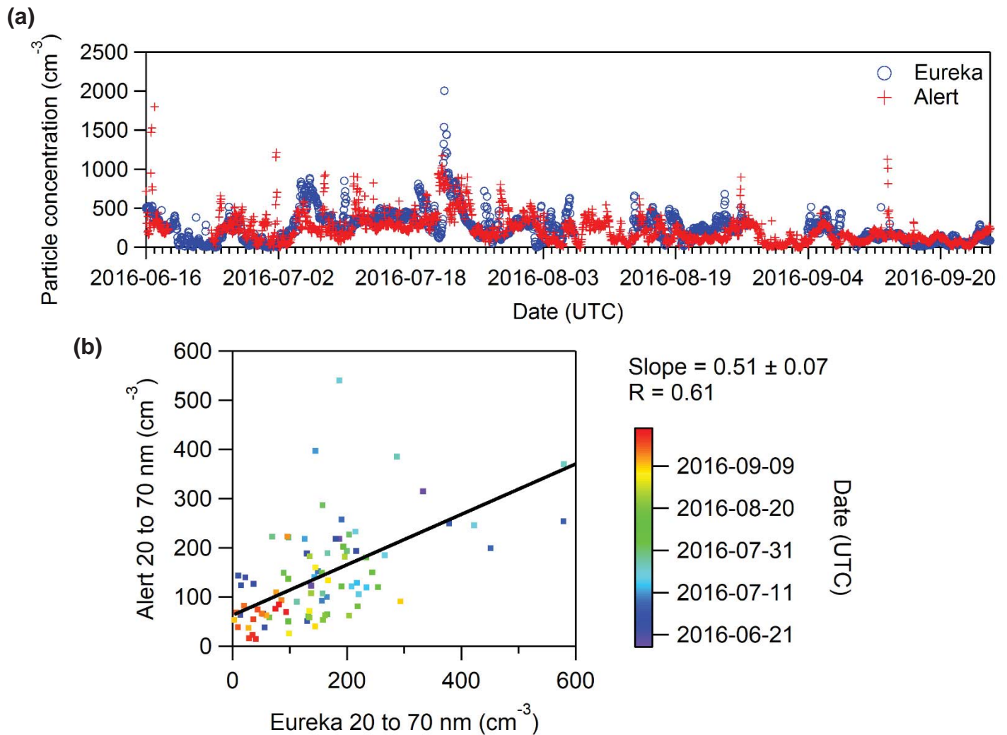
Figure 2. Total hourly particle number concentrations measured at the PEARL RidgeLab near Eureka and in Alert during summer 2016 for sizes between 10 – 487 nm (a). Scatter plot showing the correlation of the particle number concentrations measured in Alert and near Eureka (b). Note that the data in the scatter plot correspond to daily averages of particles with diameters between 20 and 70 nm.
