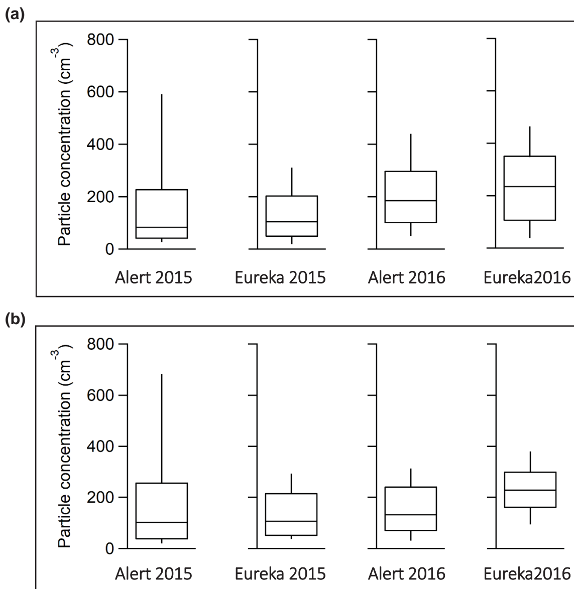
Figure 4. Box and whiskers plots of hourly particle number concentrations for diameters between (a) 10 – 487 nm, and (b) 10 – 100 nm measured during 27 Jul to 9 Sep 2015 and 2016 in Alert and at the PEARL RidgeLab near Eureka. The plots indicate the 10 th , 25 th , 50 th , 75 th and 90 th percentiles.
