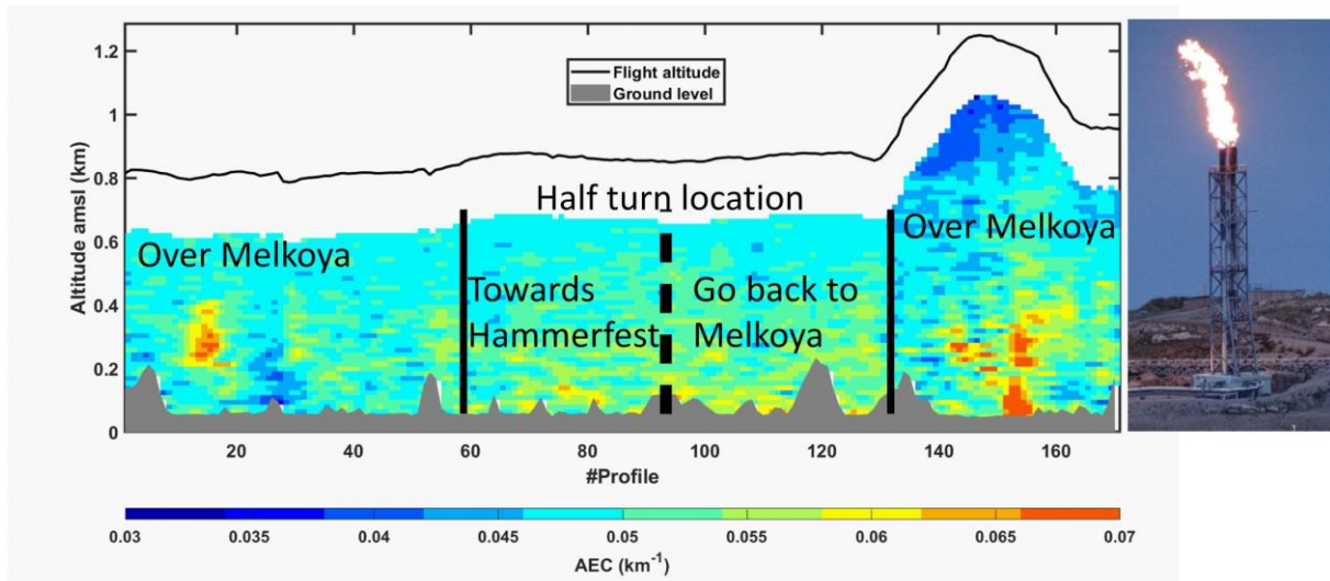
Figure 10: Left table: Vertical profile of the aerosol extinction coefficient (AEC) during the flight 4 (16 May, 2239-2324 local time) dedicated to the sampling of the Melkoya flare at 355 nm. Right picture: Flare sampled by the airborne lidar over the Melkoya platform.
