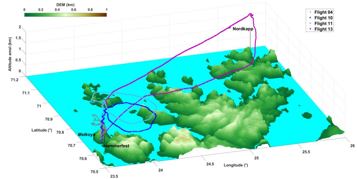
Figure 4: Flight plans used for this study: flight 04 on 16 May, flights 10 and 11 on 20-21 May, and flight 13 on 22 May (see Table 3). The flight plans are drawn over the 30 arc-second digital elevation model (DEM) GTOPO30 ( https://lta.cr.usgs.gov/GTOPO30 ).
