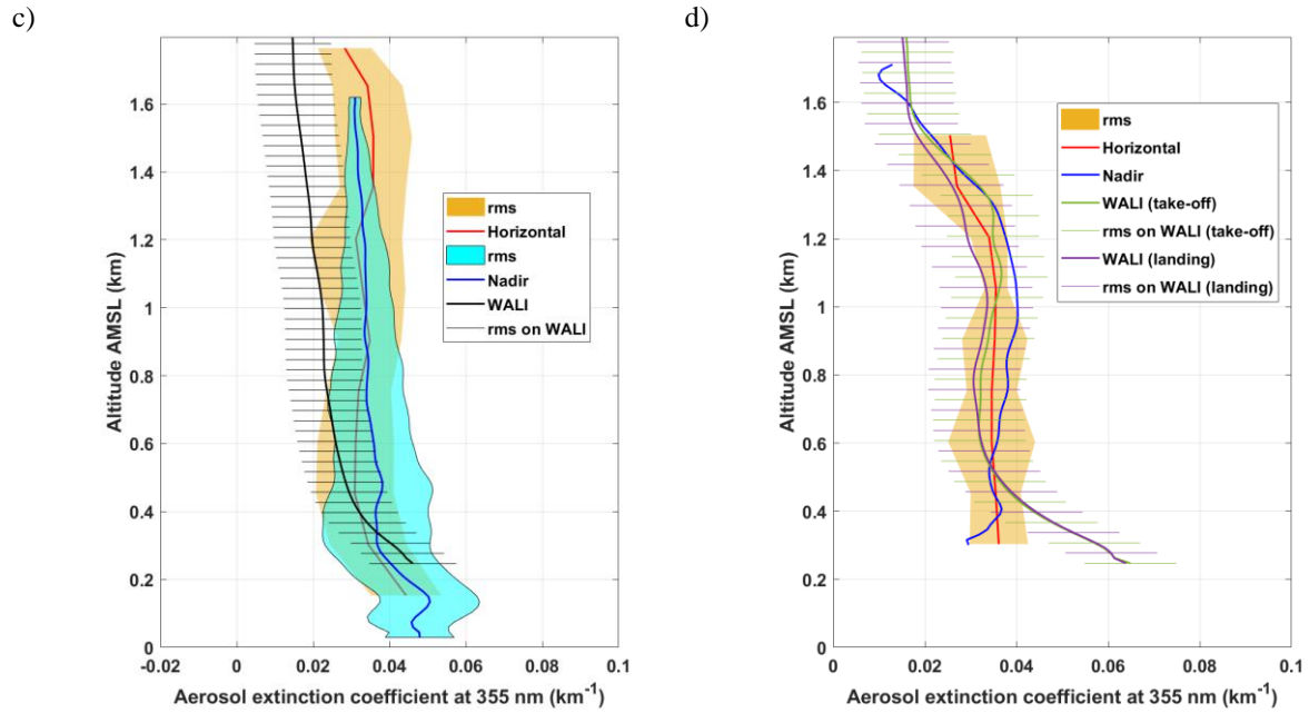
Figure 17: Vertical profiles of the AEC derived from the airborne and ground-based lidars for times corresponding to a) flight 4, b) flight 10 & 11, and d) flight 13.
