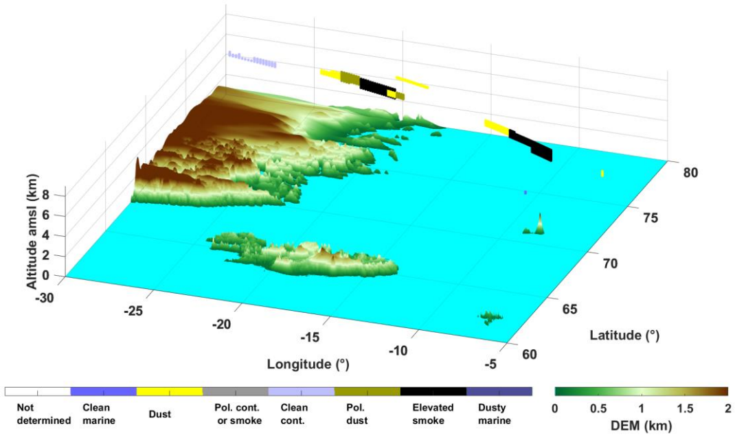
Figure 14: CALIOP-derived aerosol typing for a) the Fort McMurray on 8 May, b) the Baffin Sea on 12 May, and c) the Greenland Sea on 13 May, corresponding to the plume identified by MODIS in Figure 13.
