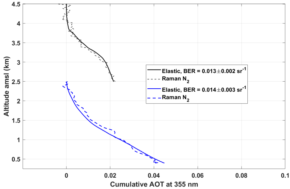
Figure 8: Cumulative aerosol optical thickness (AOT) derived from both the N 2 -Raman (dashed line) and the elastic (continuous lines) channels for the upper (black lines) and the lower (blue line) aerosol layers at 355 nm: a) 14-15 May; b) 20-21 May; c) 22-23 May.
