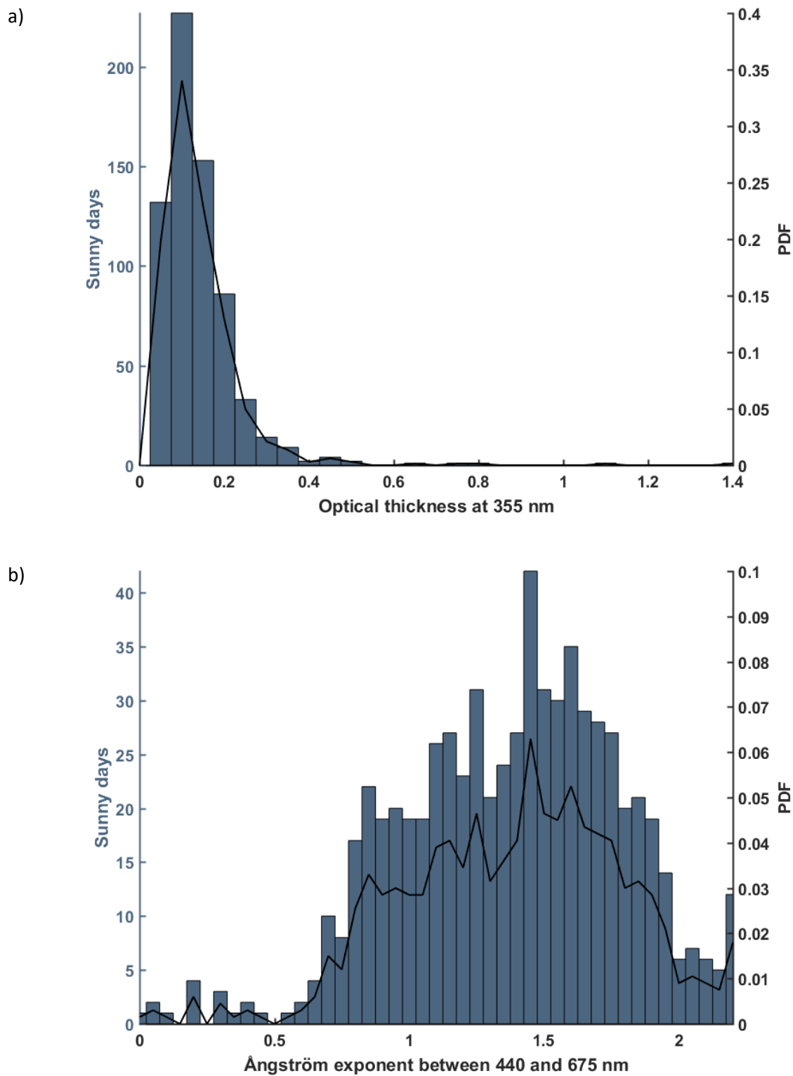
417 Figure 18: Histograms of a) the aerosol optical thickness at 355 nm and b) the Ångström exponent between 440 and 675 418 nm for the AERONET station of Andenes (69N 16E). The data are for the clear days between 2008 and 2016. The 419 probability density functions (PDF) are also given.
