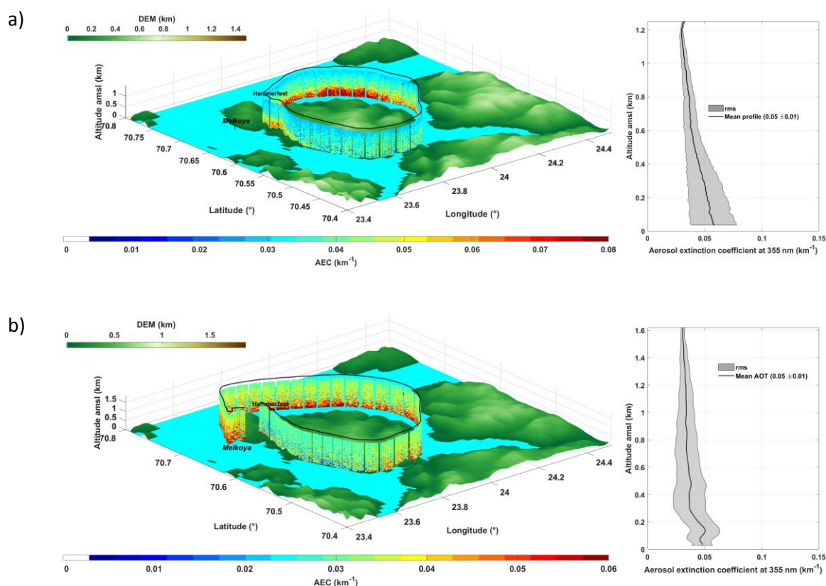
Figure 9: Vertical profiles of the aerosol extinction coefficient (AEC) derived from the lidar onboard the ULA: a) flight 10 and b) flight 11. The mean AEC vertical profiles and their dispersions are given on the right table. As in Figure 4, the flights are plotted over the digital elevation model (DEM) GTOPO30.
