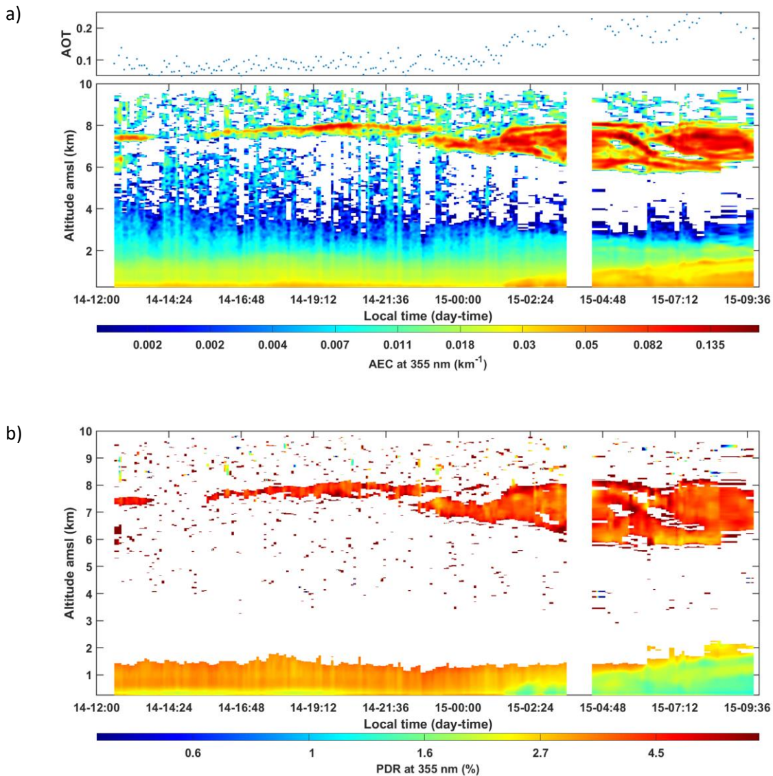
Figure 5: Temporal evolutions of a) the lidar-derived aerosol extinction coefficient (AEC) and the aerosol optical thickness (AOT); b) the particle depolarization ratio (PDR), at the wavelength of 355 nm, from 14 to 15 May, 2016.
