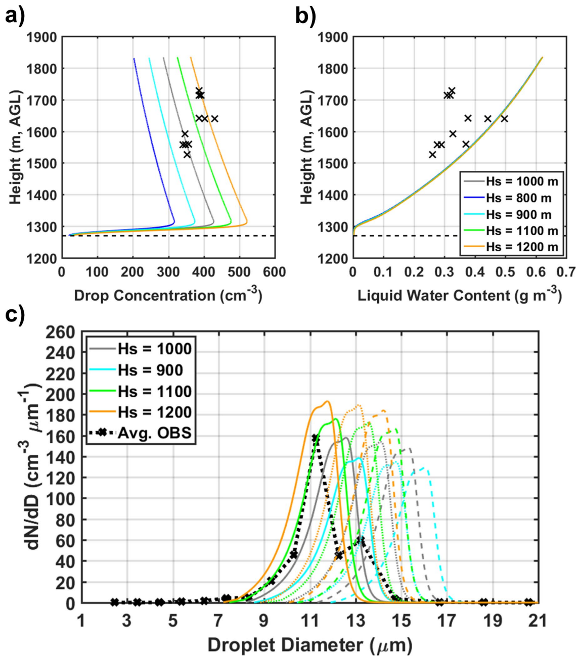
Figure 9: Sensitivity of the total drop concentration (a), LWC (b), and droplet spectra (c) at three altitudinal levels (1,500 m: solid line, 1,600 m: dotted line, and 1,700 m: dashed line) to the variations in initial aerosol concentrations at cloud base, as represented by different values of the scale height ( H_s ). In (a) and (b), the airborne observations are marked by black crosses, and the horizontal dashed line depicts CBH. The black dotted line in (c) reflects the average of five droplet spectra observed by the CDP (dotted lines in Figs. 6c and d) between 1,500 m and 1,600 m AGL.
