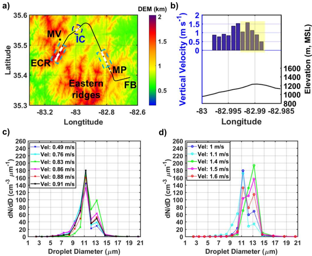
Figure 3: a) Lowest cloud transect of the UND Citation flight track on 12 June 2014. The in-cloud observations are identified as white plus signs, and MV is marked by the black asterisk. The black asterisk marks MV . For left to right in the map, ECR denotes Eastern Cherokee reservation, MP denotes Mount Pisgah, and FB denotes French Board valley. b) Updraft velocity variations of the targeted in-cloud region, denoted by IC in (a). The in-cloud samples were collected at 1-Hz (~90 m in flight distance) resolution. Cloud droplet concentrations of the in-cloud samples in IC (b) with low (0–1 m s -1 ) and high (1–2 m s -1 ) updrafts are shown in (c) and (d), respectively. The updraft velocity of each sample is indicated in the legend. Dotted lines represent the droplet spectra in the reference sub-region within IC, within yellow shade region in (b).
