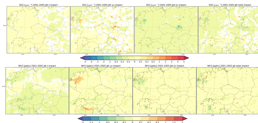
Figure 10. Same as Fig. 9 but for \text{SO}_2 (upper row) and \text{NH}_3 (lower row) in ppbv.
