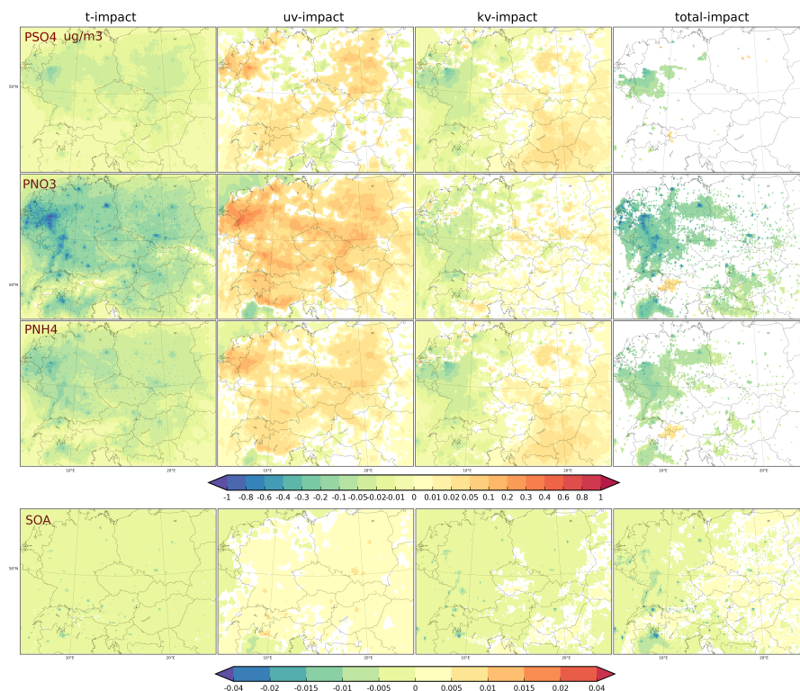
Figure 9. Impact of urban canopy meteorological forcing on (from top to bottom) \text{PSO}_4 , \text{PNO}_3 , \text{PNH}_4 and \text{SOA} average 2001-2005 JJA surface concentrations in \mu\text{g m}^{-3} . The columns from left to right correspond to temperature, wind, turbulence and the total impact. Shaded areas represent statistically significant impact on the 98% level using t-test.
