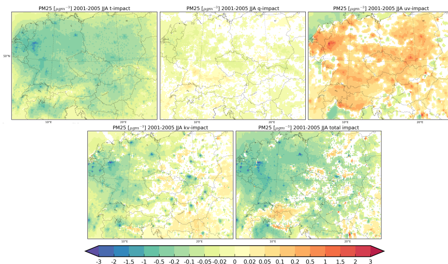
Figure 4. Impact of urban canopy meteorological forcing on \text{PM}_{2.5} surface concentrations in \mu\text{gm}^{-3} for the 2001-2005 JJA period for the (from left to right, up to down) temperature (t), humidity (q), wind (uv), turbulence (kv) and total impact. Shaded areas represent statistically significant impact on the 98% level using t-test.
