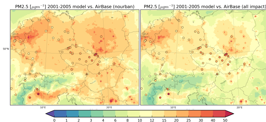
Figure 3. Absolute surface \text{PM}_{2.5} concentrations in \mu\text{gm}^{-3} averaged over the 2001-2005 JJA period for the NOURBAN experiment (i.e. without urban surface meteorological effects) and with the experiment where all urban meteorological effects are considered. Circles represent measured values from the Airbase database.
