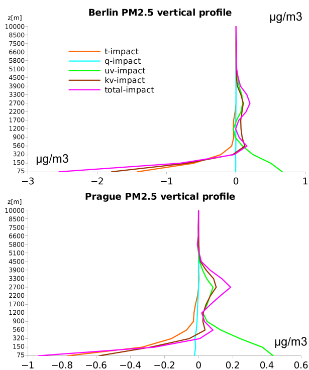
Figure 12. Impact of urban canopy meteorological forcing on the vertical profile of PM_{2.5} concentrations for two selected cities, Berlin and Prague in \mu g m^{-3} averaged over the 2001-2005 JJA period: temperature impact – orange, humidity impact – aquamarine, wind impact – green, turbulence – brown and total impact – purple). Vertical axis shows the layer interface heights in meters for the 18 CTM layers.
