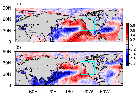
Figure 8. (a) Correlation coefficients between regional precipitation ( 43^{\circ} – 50^{\circ} N, 115^{\circ} – 130^{\circ} W) and SST variations in April for 1984–2016. (b) Correlation coefficients between March ASO ( \times -1 ) and April SST variations for 1984–2016. Dots denote significance at the 95% confidence level, according to Student’s t -test. Before performing the analysis, the seasonal cycle and linear trend were removed from the original data. ASO data are from SWOOSH, precipitation from GPCP, and SST from HadSST.
