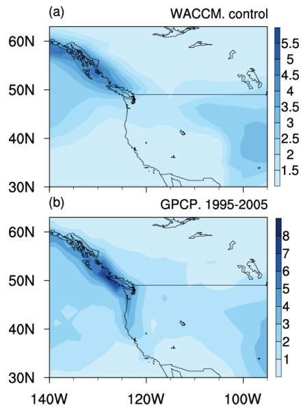
Figure 6. (a) Spatial distribution of April precipitation (mm/day) climatology in the control experiment (R1). (b) Same as (a), but precipitation from the GPCP for the period 1995–2005. For details of specific experiments, see Table 1.
