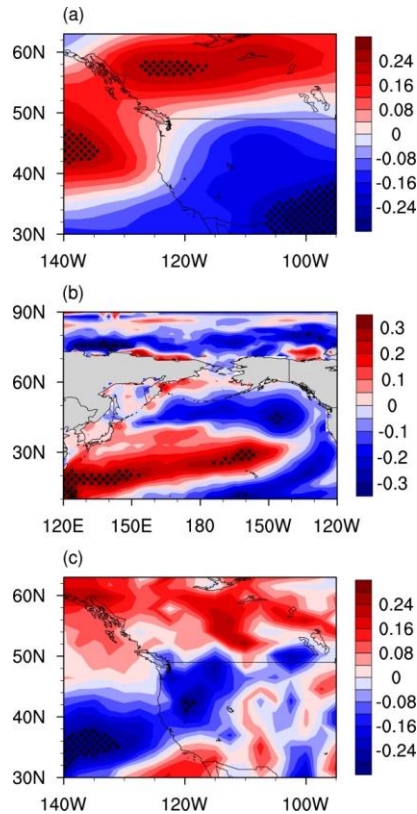
Figure R2. Correlation coefficients between the specified March ASO variations and simulated anomalies of April U (a), SST (b), and precipitation (c) for the period 1955–2005 based on the transient experiment R8. Regions above the 95% confidence level are dotted. The seasonal cycle and linear trend were removed from all quantities before correlation.
