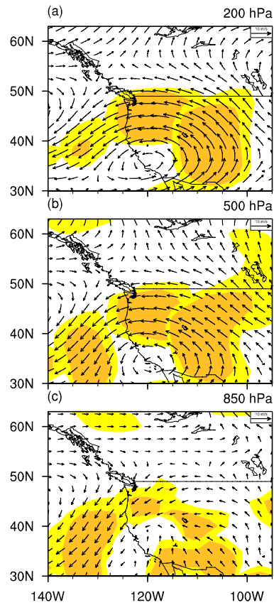
Figure 4. Differences in composite April winds (vectors, m/s, from NCEP2) between positive and negative ASO anomaly events at 200 hPa (a), 500 hPa (b), and 850 hPa (c) for 1984–2016. Colored regions are statistically significant at the 90% (light yellow) and 95% (dark yellow) confidence levels. The seasonal cycle and linear trend were removed from the original dataset. The ASO anomaly events are selected based on Table 2.
