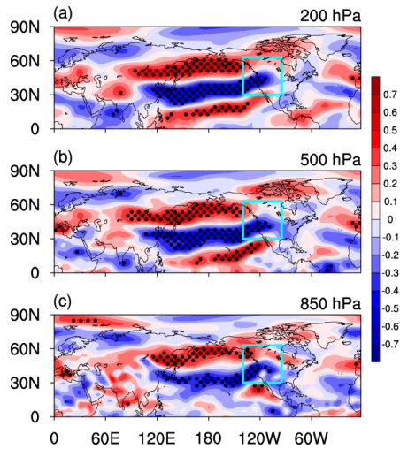
Figure 3. Correlation coefficients between March ASO index and April zonal wind variations (m/s, from NCEP2) from 1984 to 2016 at 200 hPa (a), 500 hPa (b), and 850 hPa (c). Dots denote significance at the 95% confidence level, according to Student's t -test. Blue square is the area shown in Fig. 1. Before performing the analysis, the seasonal cycle and linear trend were removed from the original datasets.
