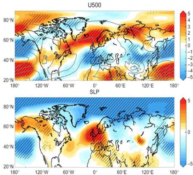
Figure R4. Figure 3 of Ivy et al. (2017). Differences (colors) in March–April zonal wind at 500 hPa ( \text{m s}^{-1} ) and sea level pressure (hPa) from MERRA between years with low March ozone and years with high March ozone. The contour lines show the climatological mean winds in the top panel; contours are every 5 \text{ m s}^{-1} ( . . . , -10, -5, 5, 10, . . . ). Hatching denotes differences that are statistically significant at the 95% level.
