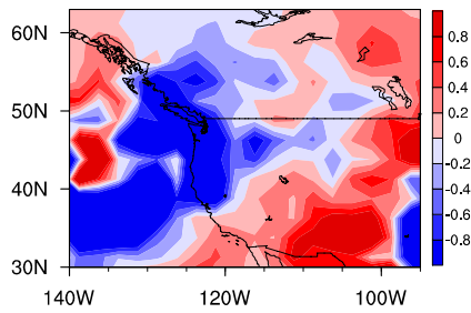
Figure R8. Differences in composite April precipitation anomalies between positive and negative ASO anomaly events during ENSO neutral years in 1984–2016. The seasonal cycle and linear trend were removed from the original dataset. The ASO anomaly events are selected based on Table R1.
