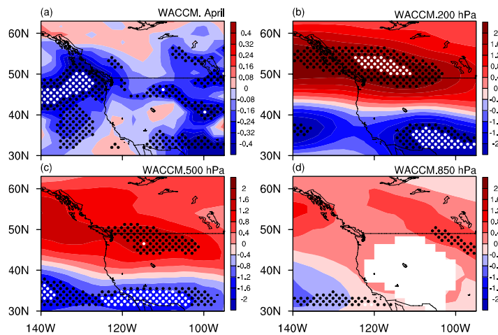
Figure R1. Differences between experiments R5 and R4 in terms of April (a) precipitation
