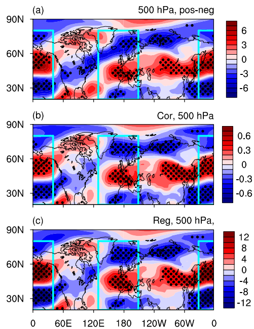
Figure R6. Same as Figure R5a, c and e, but between March ASO and March–April 500 hPa U anomalies.
