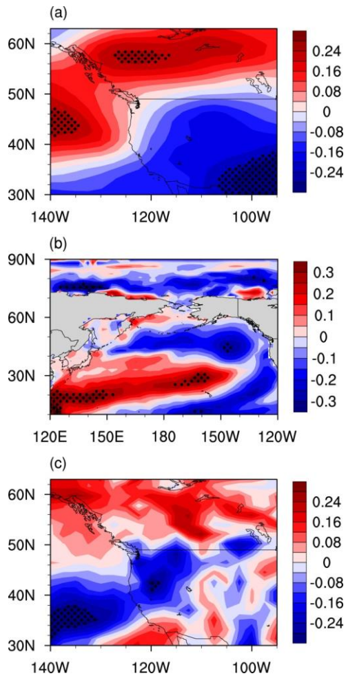
Figure RR1. Correlation coefficients between the specified March ASO variations and simulated anomalies of April U (a), SST (b), and precipitation (c) for the period 1955–2005 based on the transient experiment R8. Regions above the 95% confidence level are dotted. The seasonal cycle and linear trend were removed from all quantities before correlation.
