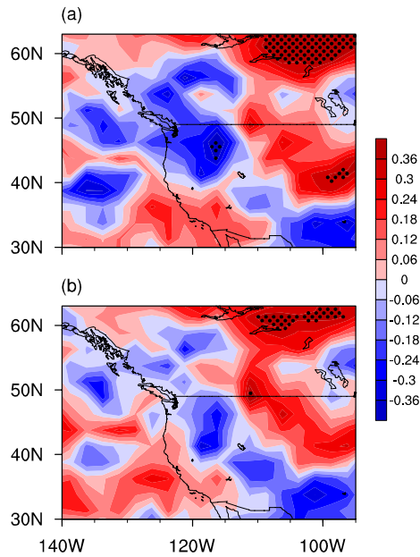
Figure R7. (a) Correlation coefficients between the March -SPV_{ASO} (the strength index of SPV is defined by Zhang et al. 2018) and April precipitation variations. (b) As for (a), but between March -SPV_{NO\_ASO} and April precipitation variations. SPV_{ASO} and SPV_{NO\_ASO} are calculated by regressing the March SPV index onto the March ASO index and removing the regressed values from the original SPV. Dots denote significance at the 95% confidence level, according to Student's t -test. The long-term linear trend and seasonal cycle in all variables were removed before the correlation analysis. The ASO data are from SWOOSH, and precipitation from GPCP.
