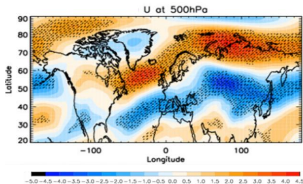
Figure R3. Figure 3 of Calvo et al. (2015). The composite differences of zonal mean zonal wind ( \text{m s}^{-1} ) at 500 hPa between the April and May averages of the LOW and HIGH ozone years during 1985–2005. Stippling indicates significant differences at the 95% confidence level.
