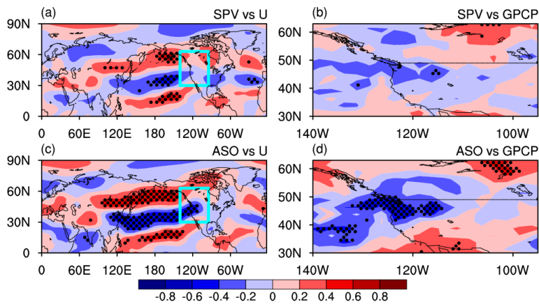
Figure 13. (a) Correlation coefficients between the February -SPV ( 10^5 \text{ K m}^2 \text{ kg}^{-1} \text{ s}^{-1} ) index defined by Zhang et al. (2018) and April zonal wind variations at 200 hPa for 1984–2016. (b) Correlation coefficients between February -SPV index and April precipitation variations. (c) and (d) As for (a) and (b), but between March ASO and April 200 hPa zonal wind and April precipitation variations. Dots denote significance at the 95% confidence level, according to Student's t -test. The long-term linear trend and seasonal cycle in all variables were removed before the correlation analysis. The ASO data are from SWOOSH, zonal wind from NCEP2, and precipitation from GPCP.
