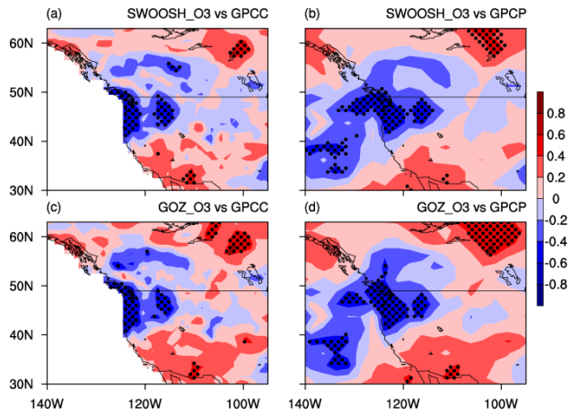
Figure 1. Correlation coefficients between March ASO and April precipitation variations calculated from SWOOSH (a, b) and GOZCARDS (c, d) ozone, and GPCC (a, c) and GPCP (b, d) rainfall for the period 1984–2016. Dots denote significance at the 95% confidence level, according to Student’s t-test. The long-term linear trend and seasonal cycle in all variables were removed before the correlation analysis.
