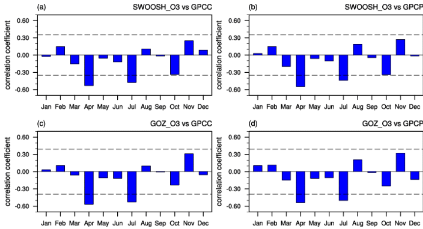
Figure 2. (a) Correlation coefficients between March ASO index and precipitation anomalies in the northwestern US ( 43^{\circ} – 50^{\circ} N, 115^{\circ} – 130^{\circ} W) for each month calculated from SWOOSH (a, b) and GOZCARDS (c, d) ozone, and GPCC (a, c) and GPCP (b, d) rainfall for the period 1984–2016. The dashed blacked lines refer to the correlation coefficient that is significance at 95% confidence level. The long-term linear trend and seasonal cycle were removed from the original datasets before calculating the correlation coefficients.
