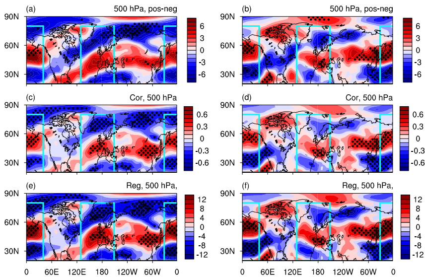
Figure R5. (a) Differences in composite March 500 hPa U wind anomalies between positive and negative ASO anomaly events. The ASO anomaly events are selected based on Table 2 in
