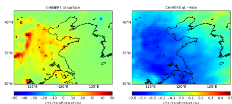
25 Figure 10: Relative difference (%) at the surface and at ~4km between CHIMERE simulation based on corrected NO x and SO 2 emissions using OMI satellite data and CHIMERE simulation based on EDGAR-HTAP-v2.2 2010 emission inventory.
