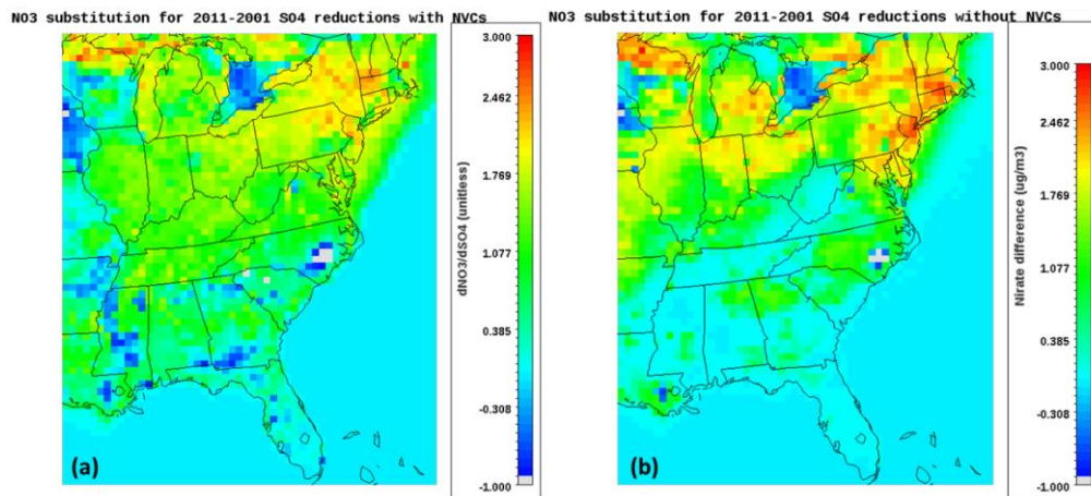
Figure 6 – CMAQ predicted nitrate substitution \left(\frac{NO_3^{2011} - NO_3^{2001}}{SO_4^{2001} - SO_4^{2011}}\right) over the decade, when NVCs are accounted for (a), and when they are removed from the thermodynamic calculations (b).
