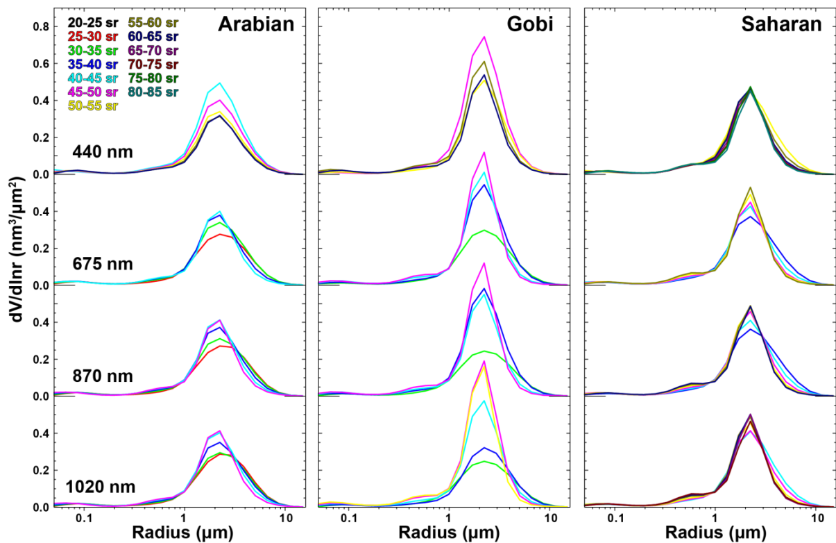
Figure 2: Mean AERONET-derived size distributions averaged according to the 5-sr intervals of S used in the histogram in Figure 4 of the original manuscript for intervals that contribute to at least 5% of the data.
