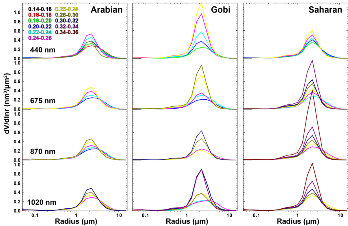
Figure 1: Mean AERONET-derived size distributions averaged according to the intervals of \delta used in the histogram in Figure 2 of the original manuscript for intervals that contribute to at least 5% of the data.
