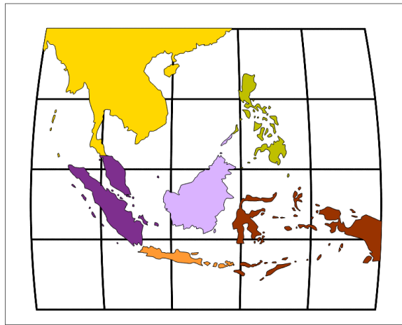
Regions for FAIE analysis
