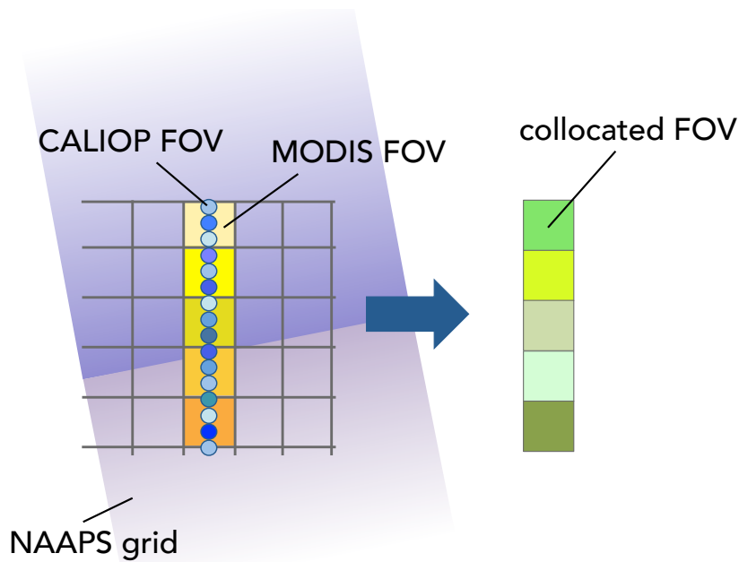
Fig. 1. Schematic showing the collocation process matching MODIS, CALIOP, and NAAPS. Multiple CALIOP fields of view (FOV) are mapped to a single MODIS FOV and averaged. Each satellite FOV is then assigned a NAAPS grid that is closest in space and time. This process is repeated for ten years of A-Train orbit to compose the CCARA dataset.
