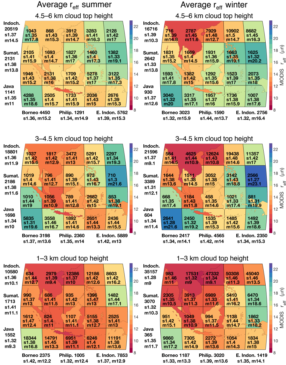
Fig. 7: Geometric means of baseline r_{\text{eff}} for each ocean grid and land region for summer (left column) and winter (right column) spanning 2006 to 2016 for three cloud height regimes. Each region is accompanied by three black bolded numbers, the first shows the number of counts in each r_{\text{eff}} population, the second is the geometric standard deviation of each population (preceded by an 's'), the third value is the median of the r_{\text{eff}} population (preceded by an 'm'). Bottom panels show clouds with tops at 1-3 km in height, middle panels show clouds at 3-4.5 km, and top panels show clouds at 4.5-6 km. The colorscale is the geometric mean of the effective radius (in microns).
