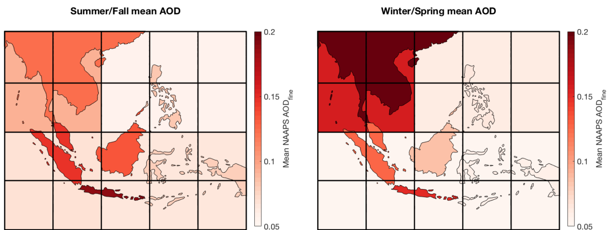
Fig. 6. Geometric means of fine mode AOD from NAAPS for the SEA domain separated into boreal summer and fall (JJASON) on the left and winter and spring (DJFMAM) on the right. Note the means are also separated by land and ocean.
