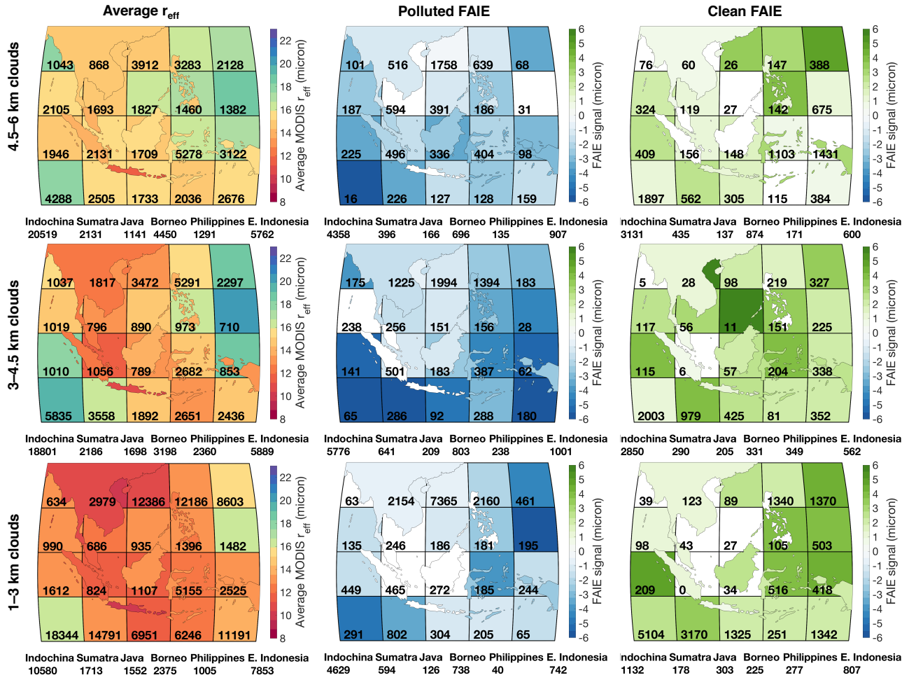
Fig. 9. Maps illustrating average baseline r_{\text{eff}} and significant polluted and clean FAIE signals. The black bolded numbers signify the count of the cloud populations. Summer months June through November are shown here. The columns from left to right show the average bulk (or baseline) r_{\text{eff}} , significant polluted FAIE, and significant clean FAIE. The rows from bottom to top show cloud top height regimes: clouds between 1-3 km, 3-4.5 km, and 4.5-6 km. Polluted and clean FAIE signals are shaded only if the significance t-test between baseline and anomalous r_{\text{eff}} populations yields a p-value < 0.01 .
