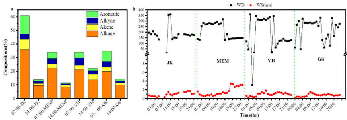
Fig.S1. Temporal variation of compositions, wind direction and wind speed on 10 th August 2017
