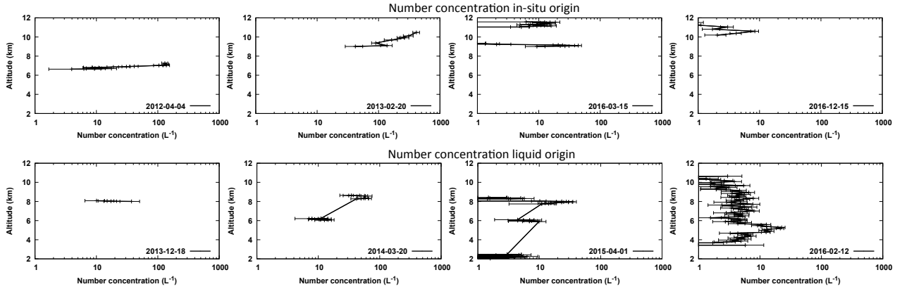
Figure 8. Number concentration as a function of altitude for all measurement days (in-situ origin top and liquid origin bottom)
