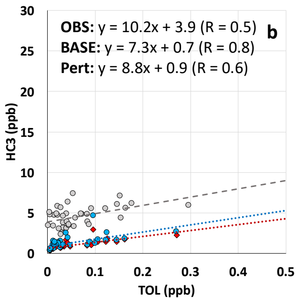
5 Figure 10. Scatter plot of HC3 vs. TOL concentrations along the C130 PM flights limited to measurements in the NFR and below 2000m altitude. Plot (a) shows HC3 vs. TOL (when measured ethane is greater than 2ppb) for measurements and the corresponding model values. Plot (b) shows HC3 vs. TOL (when measured ethane is less than 2ppb) for measurements and the corresponding model values. Grey circles represent measurements, red diamonds represent the Em7 (base emissions), and blue circles represent Em8 (perturbed emissions). Grey, Red and Blue lines show the best fit using least square linear regression method for observations, Em7 and Em8, respectively.
