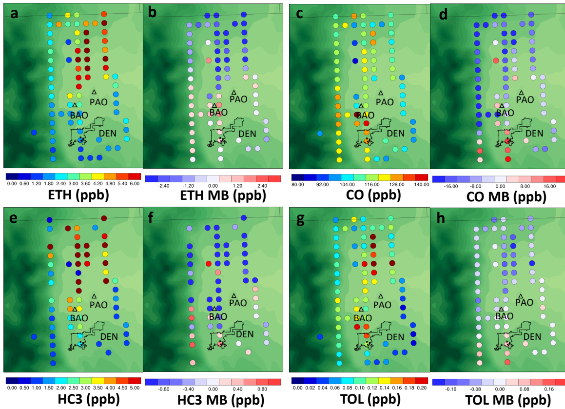
5 Figure 8. Mean and mean bias ethane concentration (a and b), CO (c and d), HC3 (e and f), and TOL (g and h) along the C130 PM flights are limited to measurements below 2000m agl and grids with more than 4 measurement points. The outline of Denver county and the locations of BAO and PAO are marked on the underlying terrain map.
