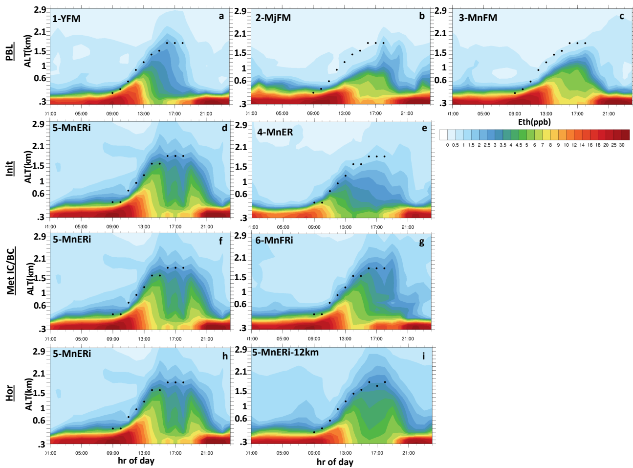
Figure 3 Cross section of modeled ethane at PAO and measured PBL height (black dots) averaged from August 1 to 10, 2014
