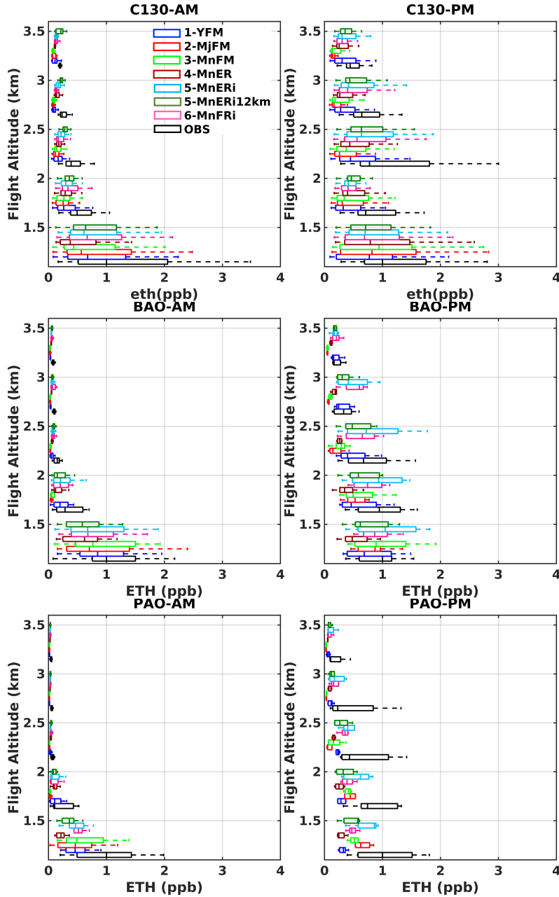
Figure 1 vertical ethane concentration distribution normalized to the measured surface ethane concentration at the surface
