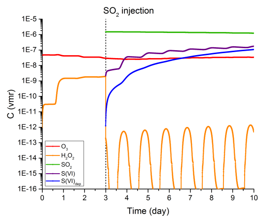
Figure 5. Time evolution in the gas-phase concentrations of SO_2 , its tropospheric oxidants and produced and deposited sulphates during S2. During S2 simulation the concentration of injected SO_2 drops from 1.5 ppmv to a final value of 1.2 ppmv.
