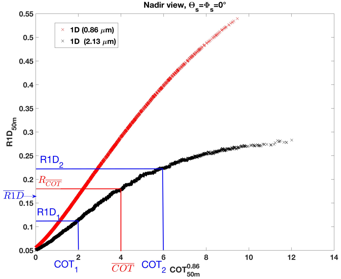
Figure 3. 1D reflectances ( R1D_{50m} ) as a function of the 50 m optical thickness at 0.86 \mu m ( COT_{50m}^{0.86\mu m} ) for channels centered at 0.86 \mu m (red) and 2.13 \mu m (black) for nadir view and overhead Sun. \overline{R1D}_1 and \overline{R1D}_2 represent the reflectances corresponding to the optical thicknesses COT_1 and COT_2 , respectively, and \overline{COT} is their averaged value. Because of the non-linearity between R1D and COT , the average reflectance \overline{R1D} is smaller than the reflectance of the average optical thickness R_{\overline{COT}} .
