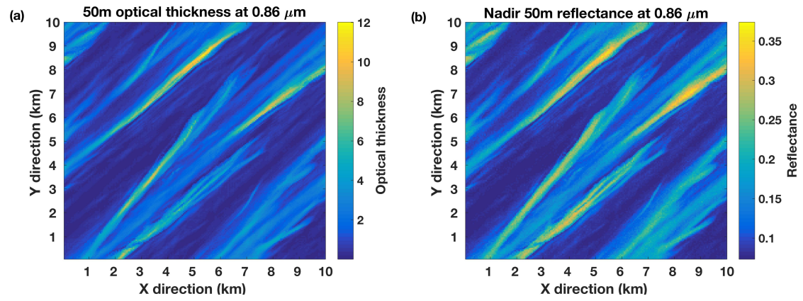
Figure 2. (a) Optical thickness field at 0.86 \mu m and (b) solar reflectance field at 0.86 \mu m at a spatial resolution of 50 m, with nadir view and overhead Sun.
