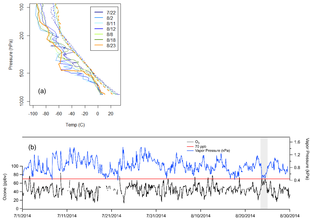
10 Figure 15. a) Denver soundings ( http://weather.uwyo.edu/upperair/sounding.html ) from high O 3 days, showing surface temperature (dashed lines) and dew point (solid lines). b) Measured O 3 concentration and water vapour at ROMO-LP during the study period. The event from August 23 is highlighted with grey shading.
