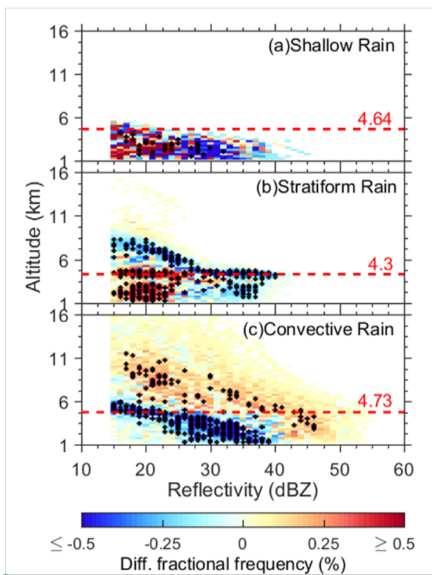
Figure 5. The differences of normalized contoured frequency by altitude diagram ( \Delta NCFAD) showing the difference in occurrence frequency for detected rain echoes (polluted minus clean) for (a) shallow, (b) stratiform, and (c) convective regimes. Data are from TRMM PR retrievals made during 2007-2012. The horizontal red dashed lines show the freezing level and the black crosses mark grid points where the difference exceeds the 95% significance level ( p < 0.05 ) according to the Pearson's \chi -square test.
