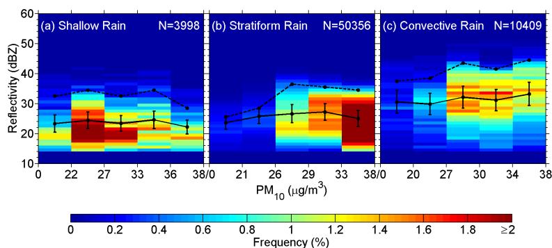
Figure 4. Joint occurrence frequency of PM_{10} - Z pair for (a) shallow, (b) stratiform, and (c) convective rain regimes respectively. Z is acquired from TRMM 2A23 products for altitudes ranging from 1 km to 5 km during the period 2007-2012. The top 1% (mean) with respect to occurrence frequency for each PM_{10} concentration bin is represented by dashed (solid) black lines. The total number of Z values ( N ) used for the calculation of frequency is shown in the upper-right corner of each panel.
