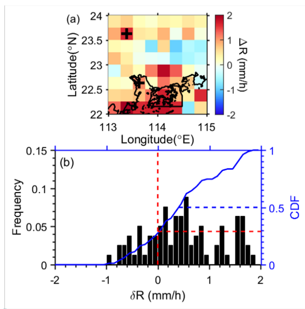
Figure 3. (a) Distribution of the differences in precipitation intensity (polluted minus clean conditions, mm/h) over the PRD region. The black dots show grid boxes for which the difference exceeds the 95% significance level ( p < 0.05 ) according to the two-tailed Student's t-test. (b) Histogram showing the occurrence frequency (OF) and its cumulative distribution frequency (CDF) of precipitation intensity differences between polluted and clean conditions. The threshold value used to discriminate between clean and polluted atmospheric conditions corresponds to lowest and highest third of the PM_{10} concentration averaged over the PRD region, respectively. The points where blue and red dashed lines cross correspond to cumulative probabilities of 29%.
