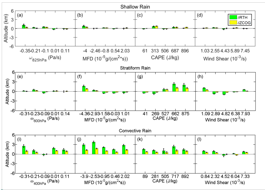
Figure 8. The differences of rain top height ( \Delta RTH ) and ZCOG ( \Delta ZCOG ) between polluted and clean conditions as a function of different meteorological conditions. (a) \omega at 825hPa pressure level, (b) MFD, (c) CAPE, and (d) vertical wind shear for shallow regime; (e) \omega at 600 hPa pressure level, (f) MFD, (g) CAPE, and (h) vertical wind shear for stratiform regime; (i) \omega at 400hPa, (j) MFD, (k) CAPE, and (l) vertical wind shear for convective regime. Data are from 2007-2012. Note that negative \omega refers to upward motion. Red and blue colors represent polluted and clean cases, respectively. The vertical error bars represent one standard deviation. Each bin in a particular panel is equally-spaced and labeled by its average value.
