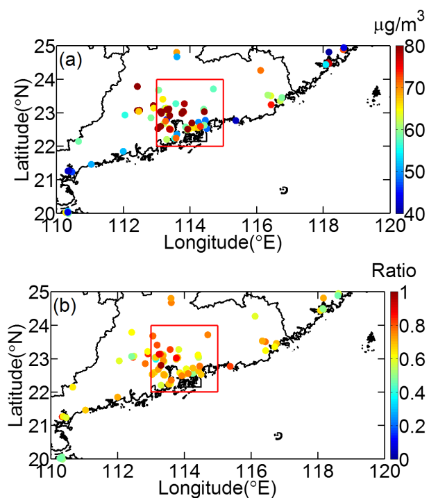
Figure 1. Spatial distributions of (a) ground-based mean PM 10 (in µg/m 3 ) and (b) the ratio of mean PM 2.5 to mean PM 10 simultaneously measured for the period from November 2013 to October 2014. The red box outlines the PRD region, the dots show the locations of the PM measurement sites.
