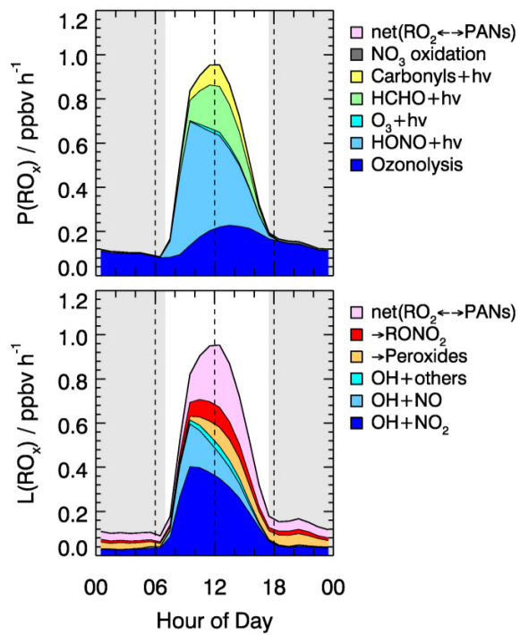
5 Figure 8. Hourly averaged primary sources and sinks of RO x radicals derived from model calculations for all episodes. The grey areas denote nighttime.
