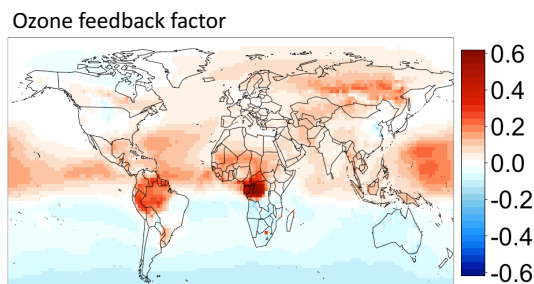
Figure 9: Ozone feedback factor ( f ) arising from the coupling between surface ozone (JJA mean) and leaf area index (LAI). A value of 0 < f < 1 indicates a positive feedback (self-amplification of surface ozone), and a value of f < 0 indicates a negative feedback (self-dampening of surface ozone).
