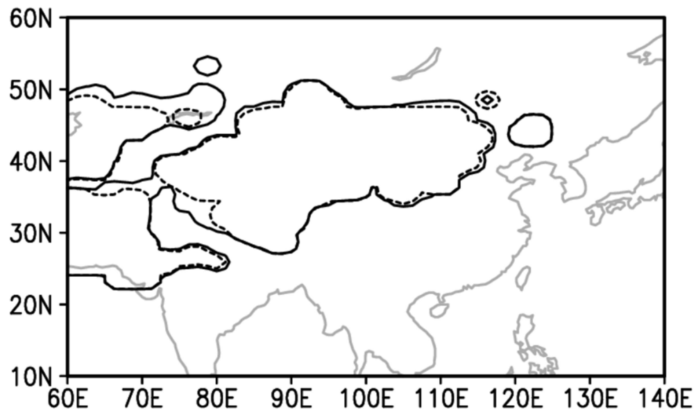
Figure S2, Dust source area defined as emission flux > 0 kg/m 2 /s with Case 1 (Real line) and Case 2 (dotted line).
