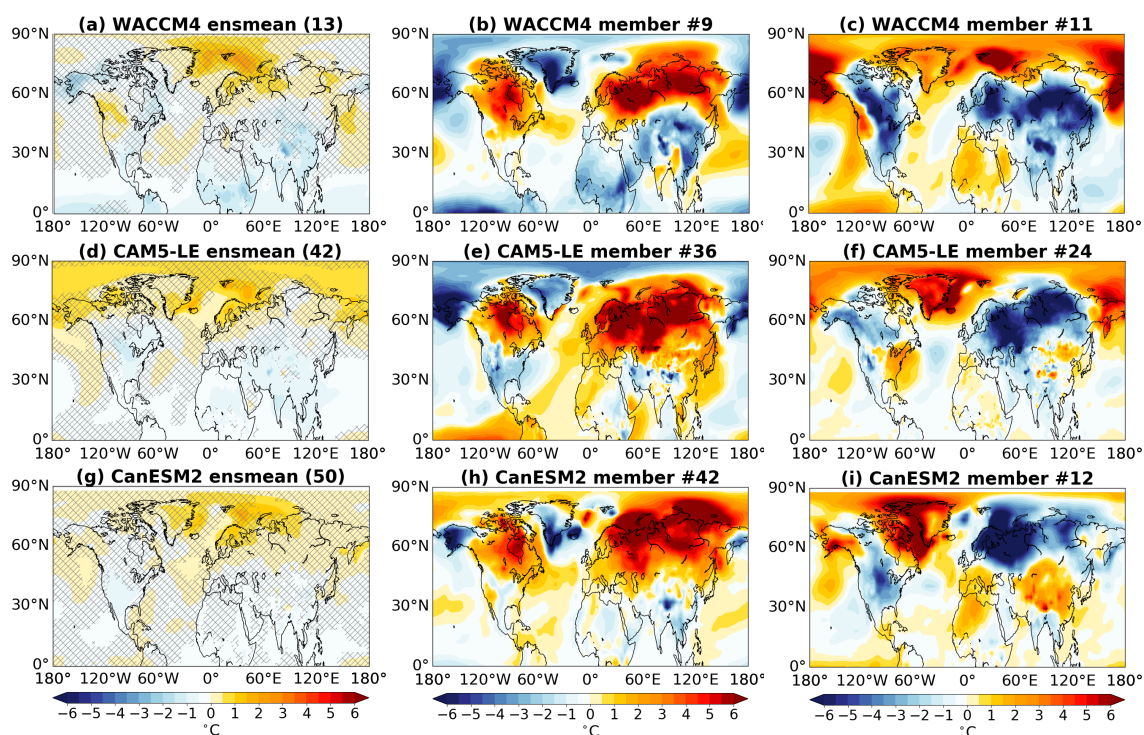
Figure 3. Wintertime surface air temperature anomalies (in °C) as simulated by WACCM4 (top row), CAM5-LE (middle row) and CanESM2 (bottom row) following the 1991 Mt. Pinatubo eruption. Left column: the ensemble mean for each model (with the number of ensemble members in parentheses), and hatching over areas where the anomalies not significant at the 95% confidence level. Middle column: individual members exhibiting extreme warming over the NH continents for each model. Right column: individual members exhibiting extreme cooling.
