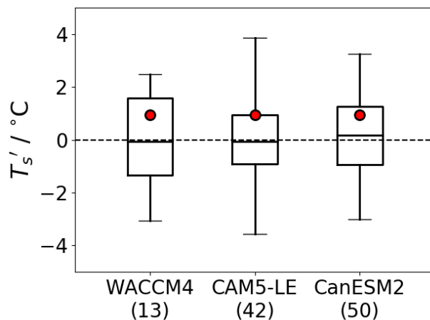
Figure 4. Box and whisker plots of simulated surface temperature anomaly (in °C) over Eurasia (40-70N, 0-150W) in the first post-Pinatubo winter (1991-92) relative to the reference period (1985-1990). The horizontal line inside each box denotes the ensemble mean; the lower and upper limits of each nbox denote the 25th and 75th percentile values, respectively; the whiskers span the full range of the ensemble members. For comparison, the red circles denote the value calculated from the ERA-Interim reanalyses.
