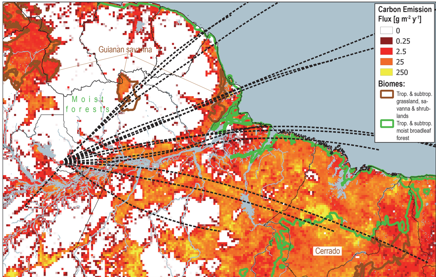
Figure 16. Map of the ATTO-relevant eastern Amazon Basin ( \text{ROI}_{\text{foot}} ) combining the backward trajectory (BT) data with (i) a GFAS-derived map of the average fire-related carbon emission flux within time period from 2003 to 2017 according to Kaiser et al., (2011) and (ii) a biome classification according to Olson et al., (2001) (see Fig. 10a). The pixel size of the fire map equals \sim 11 km. The BT data is represented as center lines of the 15 BT clusters (black dashed lines, see Fig. 4). For comparison, Fig. S17 shows a fire map with higher spatial resolution ( \sim 1 km resolution), which shows the same geospatial patterns.
