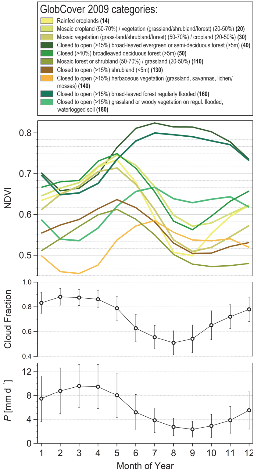
Figure 13. Seasonal cycles in normalized difference vegetation index (NDVI) for the ROI_{foot} -relevant GlobCover 2009 categories as specified in Table 3. The NDVI data is provided as monthly means. Seasonal cycles for precipitation and cloud cover, which indirectly represents solar radiation, have been added and are shown as monthly means with error bars representing one standard deviation.
