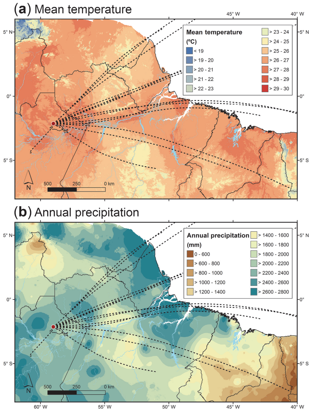
Figure 9. Map of the ATTO-relevant eastern Amazon Basin ( ROI_{foot} ) combining the backward trajectory (BT) data with GIS data layers of (a) mean temperature and (b) annual precipitation, both obtained from the WorldClim database (Hijmans et al., 2005; worldclim.org). The BT data is represented as center lines of the 15 BT clusters (black dashed lines, see Fig. 4).
