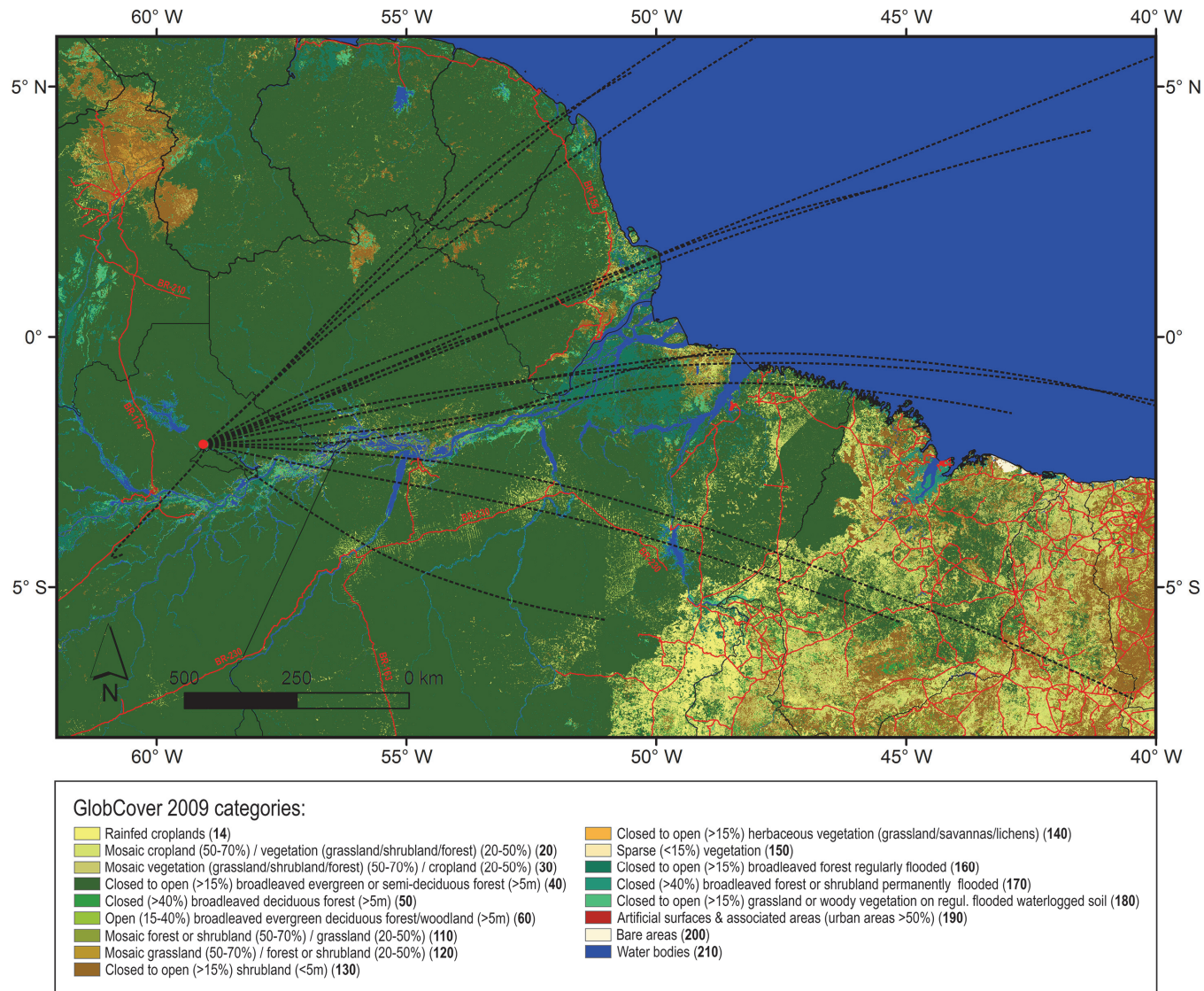
Figure 11. Map of the ATTO-relevant eastern Amazon Basin ( ROI_{foot} ) combining the backward trajectory (BT) data with GIS layers of a land cover map based on the GlobCover 2009 data (Arino et al., 2008) and a map of major roads. The BT data is represented as center lines of the 15 BT clusters (black dashed lines, see Fig. 4).
