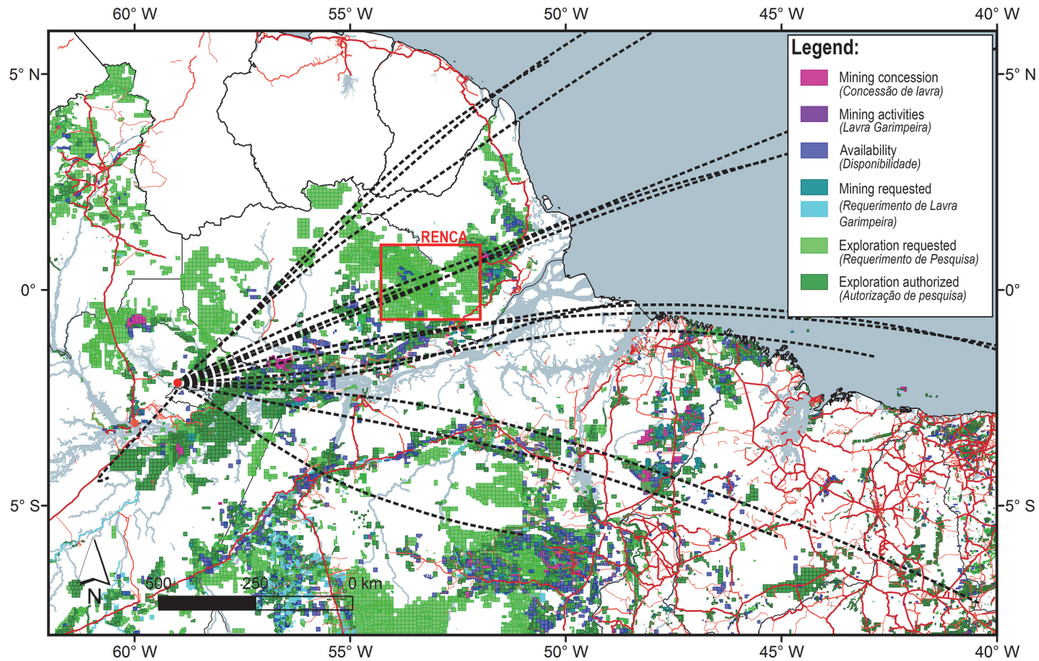
Figure 20. Map of the ATTO-relevant eastern Amazon Basin ( ROI_{foot} ) combining the backward trajectory (BT) data with GIS data on mining activities. The legend specifies several categories of mining activities according to SIGMINE (see Sect. S1.1). The BT data is represented as center lines of the 15 BT clusters (black dashed lines, see Fig. 4).
