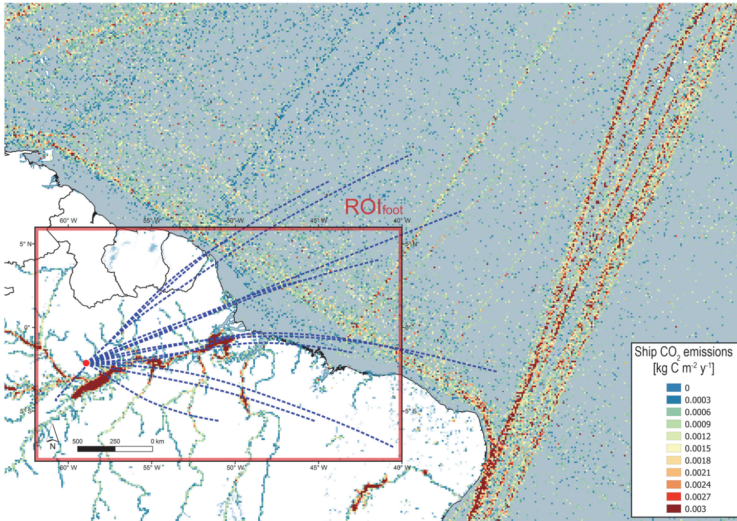
Figure 19. Map of eastern Amazon Basin, including ROI foot , and western Atlantic Ocean in combination with ship tracks. Ship tracks are represented by modelled shipping-related CO 2 emission according to Asefi-Najafabady et al. (2014). The BT data is represented as center lines of the 15 BT clusters (blue dashed lines, see Fig. 4).
