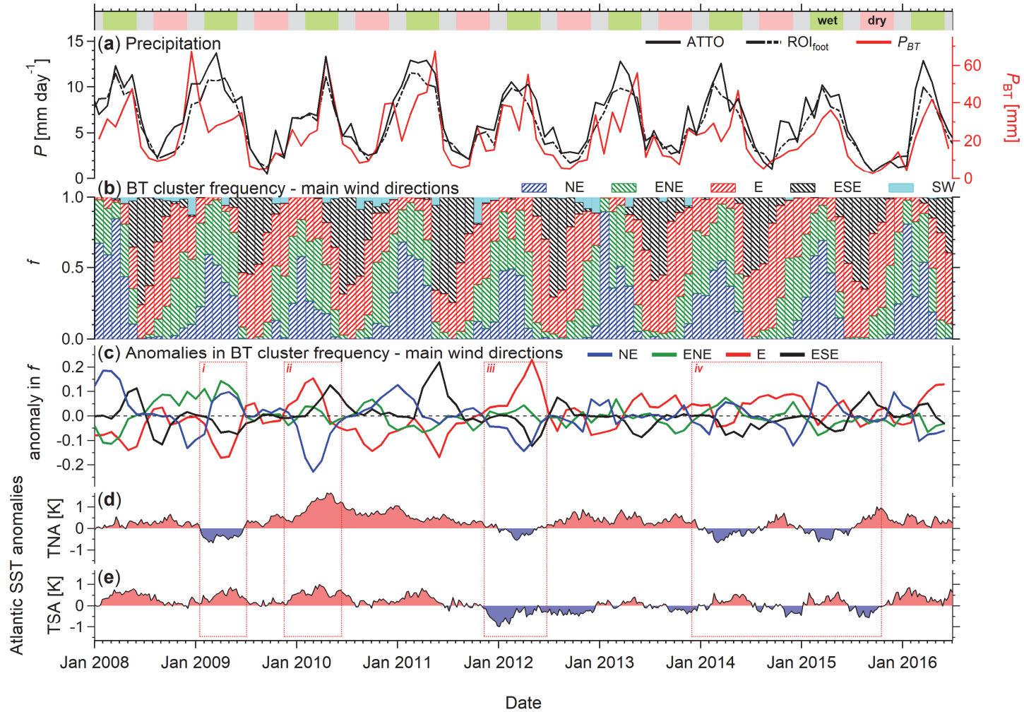
Figure 6. Multiyear variability and anomalies in BT advection in relation to Atlantic sea surface temperatures. (a) Area-averaged precipitation rates, P , for the \text{ROI}_{\text{ATTO}} and continental part of the \text{ROI}_{\text{foot}} (for both, see Fig. 4). Furthermore, cumulative precipitation along 3-days BTs tracks, P_{\text{BT}} , is shown. All precipitation data is shown as monthly means. (b) Frequency of occurrence, f , of main directions of BT advection from NE, ENE, E, ESE, and SW. Data is shown as monthly means. (c) Anomalies in frequency, f , of main directions in BT advection. Data is shown as monthly means. Red boxes i , ii , iii , and iv highlight examples of pronounced anomalies in f . (d) and (e) Anomalies in sea surface temperature of tropical north Atlantic (TNA) and tropical south Atlantic (TSA). Colored shading in top row represents aerosol-related definition of seasonality in ATTO region according to M. Pöhlker et al. (2016).
