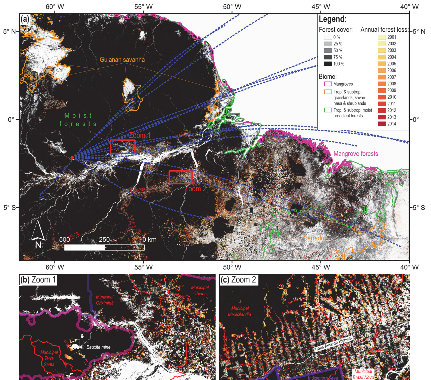
Figure 14. Map of the ATTO-relevant eastern Amazon Basin ( ROI_{foot} ) combining the backward trajectory (BT) data with GIS layers of (i) a forest cover map of the year 2000, according to Hansen et al. (2013), (ii) a map on annual forest loss within the period 2001-2014 (Hansen et al., 2013), and (iii) contour lines representing the dominant biomes (see Fig. 10a). The BT data is represented as center lines of the 15 BT clusters (blue dashed lines, see Fig. 4). A map of the ROI_{foot} with afore mentioned GIS layers is shown in (a), whereas (b) and (c) zoom into two smaller regions of particular interest.
