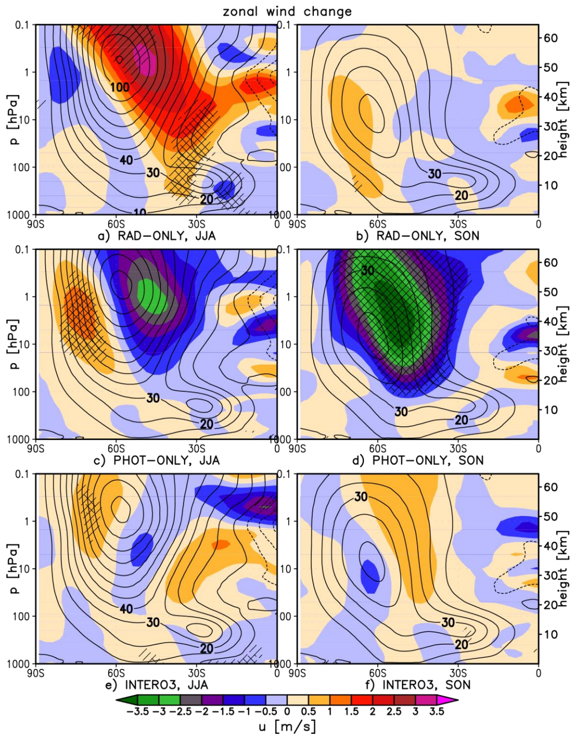
Figure 3. Shading: seasonal mean (left: JJA and right: SON) SH zonal mean zonal wind change [ \text{m s}^{-1} ] between SMAX and SMIN for (a-b) RAD-ONLY, (c-d) PHOT-ONLY and (e-f) INTERO3. Single and double hatching indicates statistical significance at the 90% and 95% confidence level, respectively (t-test). Contours show the corresponding climatological seasonal mean zonal mean zonal wind for the respective SMIN run; contour spacing is 10 \text{ m s}^{-1} .
