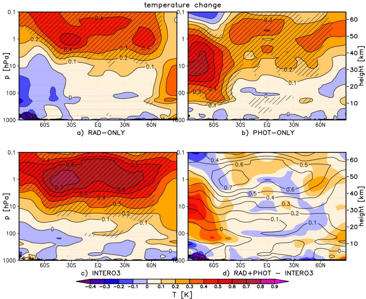
5 Figure 1. Yearly mean zonal mean temperature change [K] between SMAX and SMIN for (a) RAD-ONLY, (b) PHOT-ONLY and (c) INTERO3. Hatching in (a-c) shows regions where the response is statistically significant at the 95% level (calculated using a two-tailed Student's t-test). Shown also (d) is the difference (shading) between the sum of the single forcing responses and INTERO3 (contours, as in (c)).
