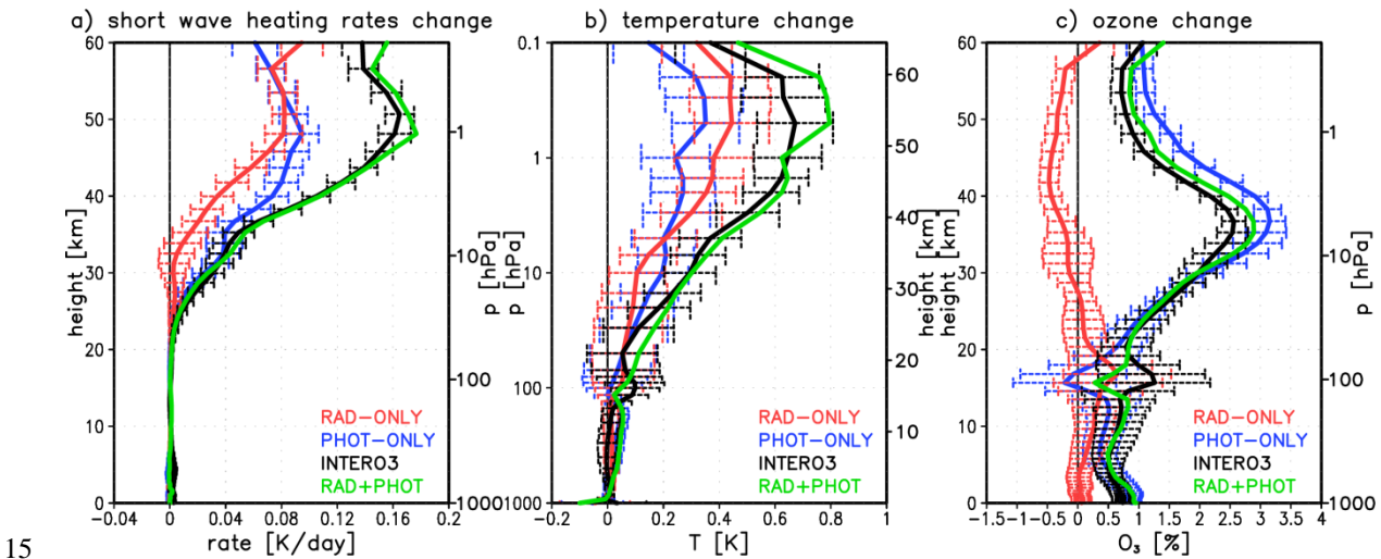
Figure 2. Yearly mean tropical average ( 25^\circ\text{N} - 25^\circ\text{S} ) change in (a) the shortwave heating rates [ \text{K day}^{-1} ], (b) temperature [K], and (c) ozone [%] between SMAX and SMIN for RAD-ONLY (red), PHOT-ONLY (blue) and INTERO3 (black), together with the associated confidence intervals ( \pm 2 standard errors). The green line indicates the sum of the RAD-ONLY and PHOT-ONLY responses.
