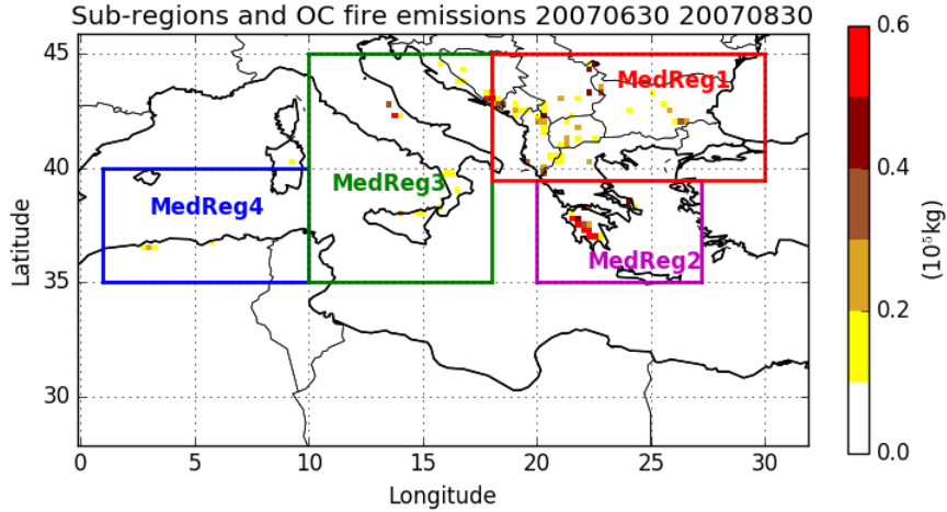
Figure 2.1. Map of the nested domain over the Mediterranean area with a spatial resolution of 0.25^\circ \times 0.25^\circ . The total organic carbon emissions ( \text{kg} \cdot (\text{grid cell})^{-1} ) from fires during the summer of 2007 are presented. The sub-regions used in this study are also indicated in colored boxes: MedReg1 (Balkan + Eastern Europe), MedReg2 (Greece), MedReg3 (Italy) and MedReg4 (Algeria).
