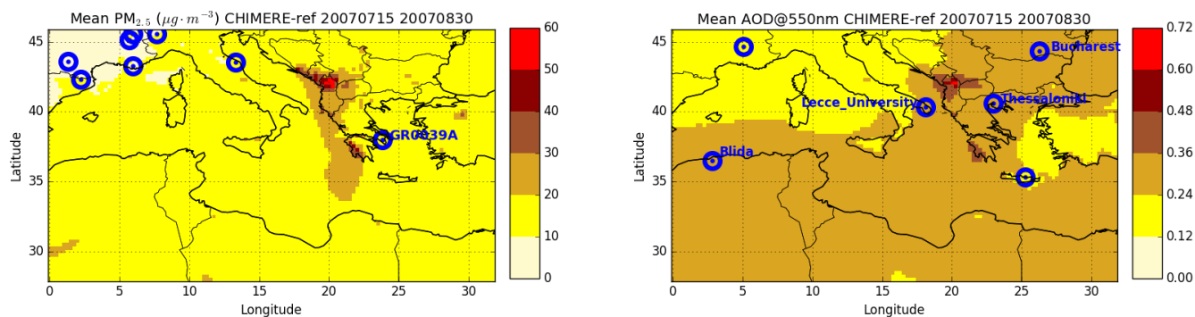
Figure B1. Daily mean surface PM 2.5 and AOD at 550 nm from the CHIMERE-ref simulation averaged over the summer of 2007 (the 8 AIRBASE and 6 AERONET stations, used in this work, are represented here in blue dots).
