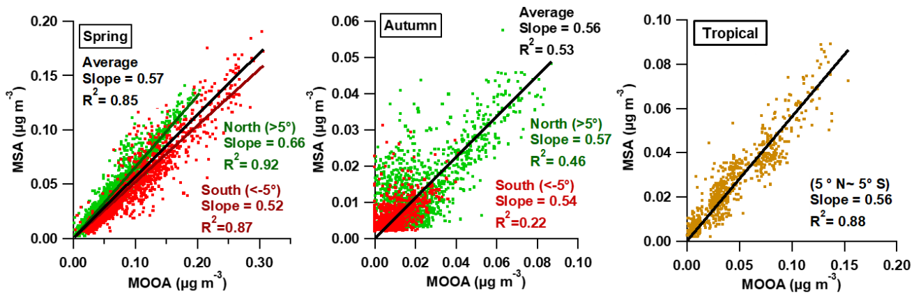
5 Figure 7 The correlations between the MSA and MOOA factor in spring and autumn over different regions of the Atlantic Ocean
