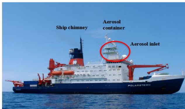
5 Figure 1. (a) Ship tracks of 4four cruises; (b) The position of the container during Polarstern cruises.
