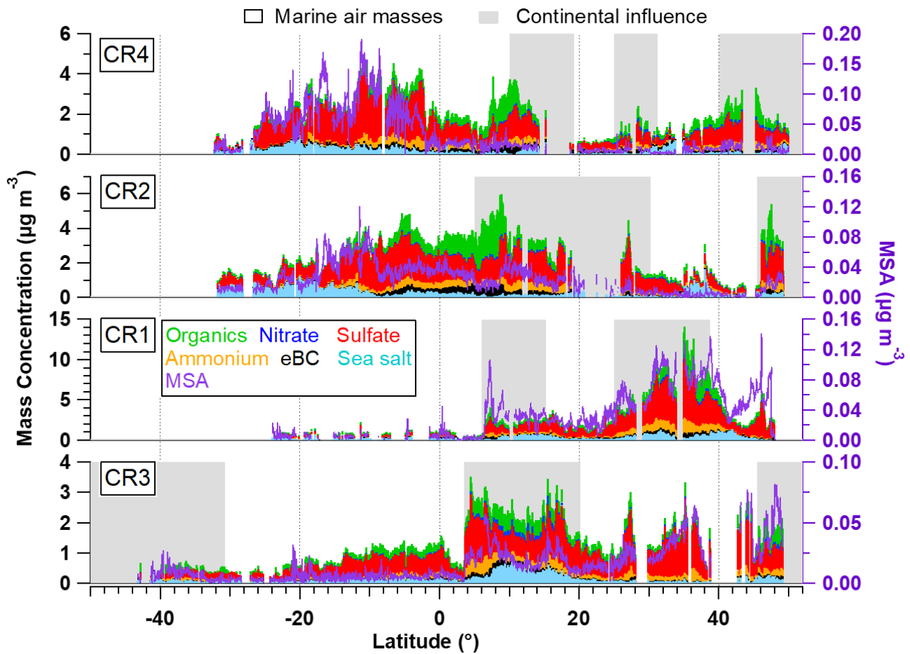
Figure 2. Latitudinal variation of organics, nitrate, sulfate, ammonium, eBC, sea salt (left axis) and MSA (right axis) during the 4four Polarstern cruises. Air masses with continental influence (grey) and originated from the ocean (blank) are marked on background. Note that CR1, CR2, and CR4 followed almost the same ship track between Bremerhaven and Cape Town, while the route of CR3 was different (from 15°N) since starting from Punta Arenas.
