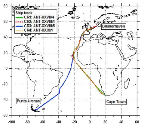
5 Figure 1. (a) Ship tracks of 4four cruises; (b) The position of the container during Polarstern cruises.
