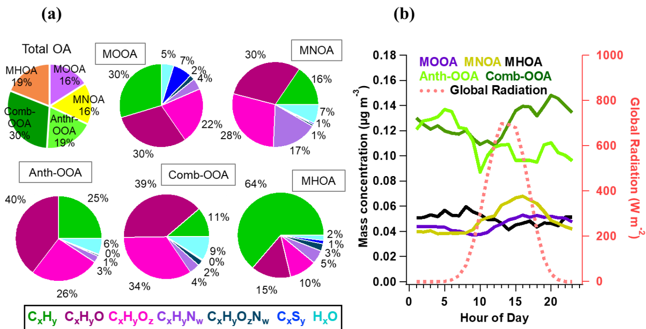
Figure 4 (a) Average mass fraction of each component in the total OA mass concentration, and the functional groups composition of each OA factor, and (b) diurnal variations of five OA factors with global radiation.
