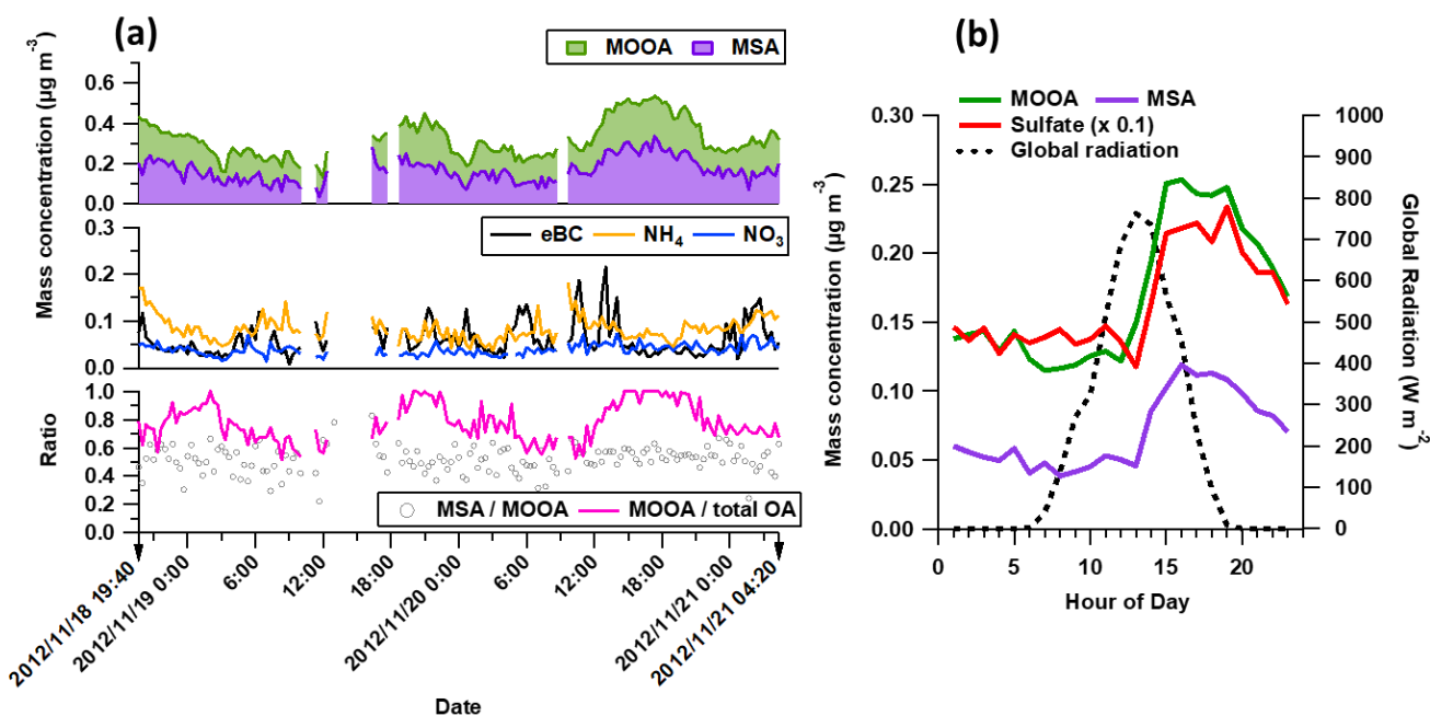
5 Figure 6 The characteristics of the MOOA dominating period: (a) time series of MOOA and MSA (top), possibly non-marine species (eBC, \text{NH}_4 , \text{NO}_3 ; middle figure), as well as the ratio between MSA and MOOA, and the mass fraction of MOOA in the total OA (bottom); (b) the diurnal variation of MOOA, MSA, Sulfate (reduced to one tenth for comparison) and the global radiation.
