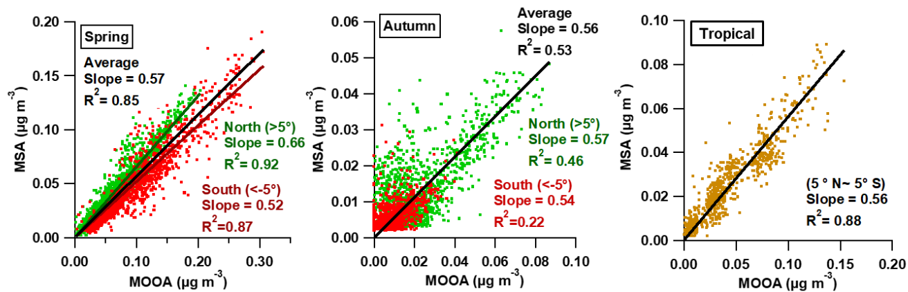
Figure 7 The correlations between the MSA and MOOA factor and MSA in spring and autumn over different regions of the Atlantic Ocean
