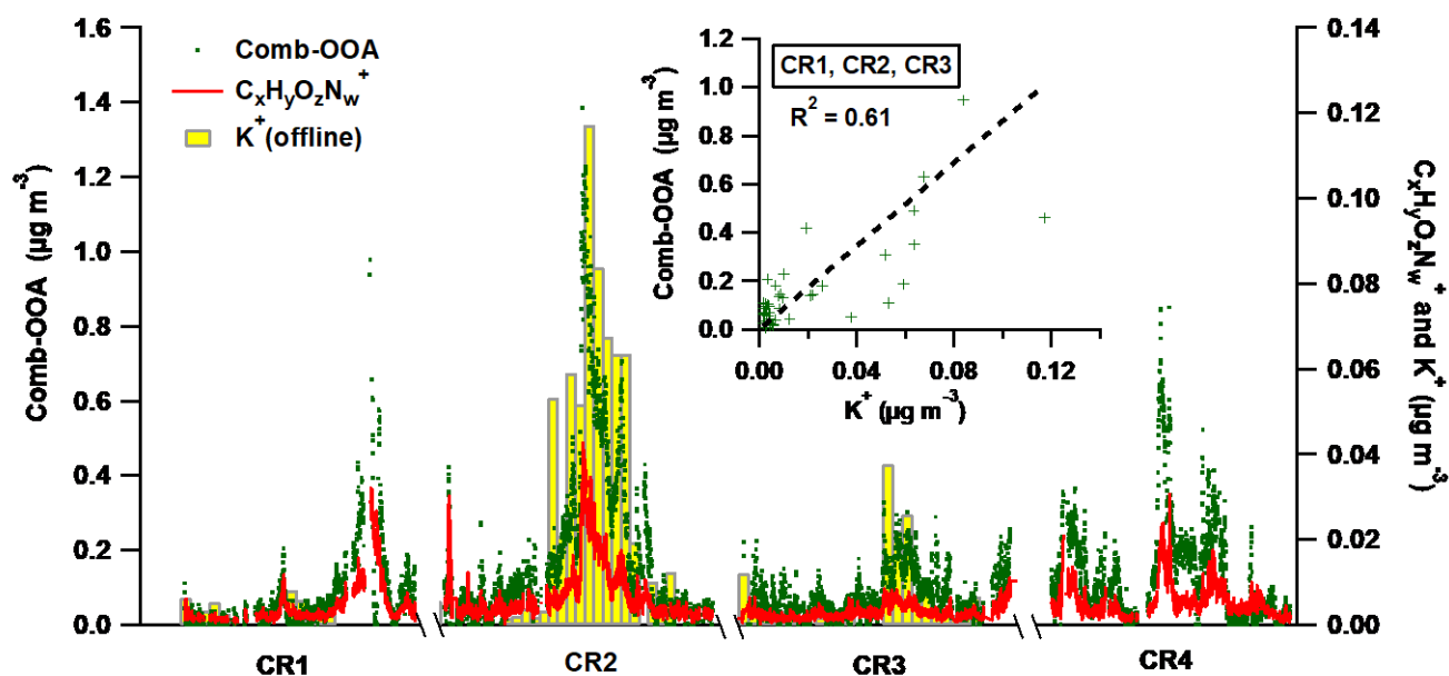
5 Figure 8 The variation of Comb-OOA (green dots ), C_xH_yO_zN_w^+ fragments (red line) and potassium ( K^+ , the yellow bar with grey box) during Polarstern cruises. Note that the 24h-average mass concentration of K^+ is obtained from offline measurements only performed during the first three cruises. The scattering plot in the sub-window provides the correlation between 24h-average mass concentration of Comb-OOA from AMS and potassium from offline measurements.
