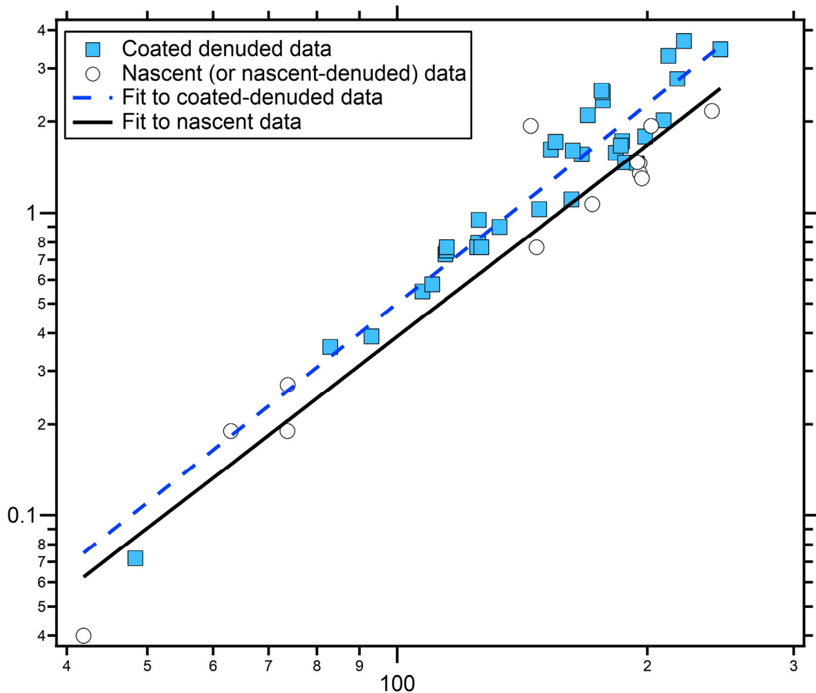
Figure S8. Fit of CPMA mass per particle as a function of the SMPS mode number-weighted mobility diameter for soot particles from the premixed ethylene flame from BC2, when the flame was sampled at 20 cm above the burner surface. The blue squares are coated denuded observations and the dashed blue line is the associated power-law fit. The white circles are nascent observations and the black line is the associated power-law fit. The data were fit to a power law function (see eqn. 8 in the main text). For nascent soot, fit parameters C and D_{f,m} were 2.40 \times 10^{-5} and 2.12, respectively, and for coated-denuded soot, fit parameters C and D_{f,m} were 1.33 \times 10^{-5} and 2.28, respectively.
