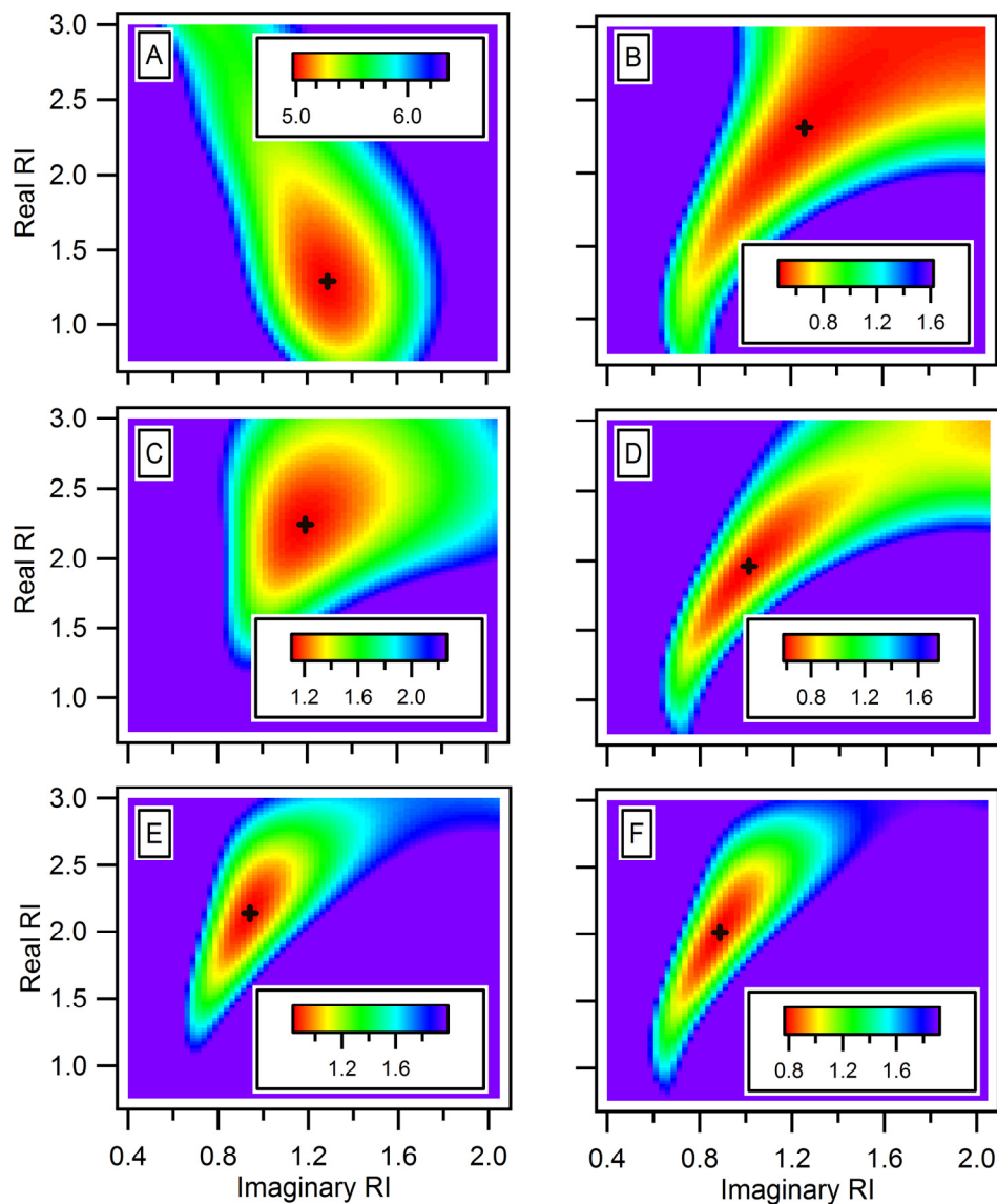
Figure S3. Image plots of the reduced \chi^2 values of Mie Theory fits to absorption for all methane flame data. The colors represent the reduced \chi^2 value at each effective refractive index. Each panel differentiates between different wavelengths. The column on the left is the fit over all size parameters and the column on the right corresponds to size parameter (x) < 0.9 . The minimum reduced \chi^2 are shown as black crosses. Panels A and B correspond to \lambda = 405 nm data, panels C and D correspond to \lambda = 532 nm data, and panels E and F correspond to \lambda = 630 nm data. Purple on the image plots indicates the region beyond 1 standard deviation of the reduced \chi^2 value ( \chi^2 + 1.11 ).
