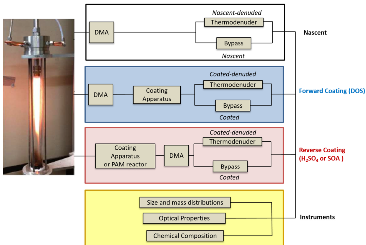
Figure S1. General experimental set-up for BC2, BC3, BC3+, and BC4, for the methane diffusion flame. Note that during BC4, particles were mass-selected with a CPMA, in addition to being size-selected.
