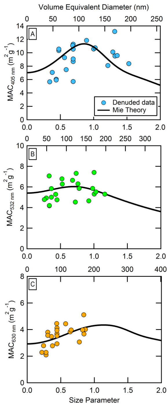
Figure S9. MACs for ethylene soot sampled 5.1 cm above the burner surface as a function of size parameter (bottom) and volume equivalent diameter (top) for (A) \lambda = 405 nm, (B) \lambda = 532 nm, and (C) \lambda = 630 .
