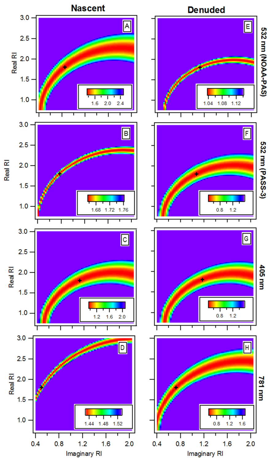
Figure S7. Same as Figure S6, except for RDG fits instead of Mie fits. Panel letters correspond to the same datasets as Figure S6.
