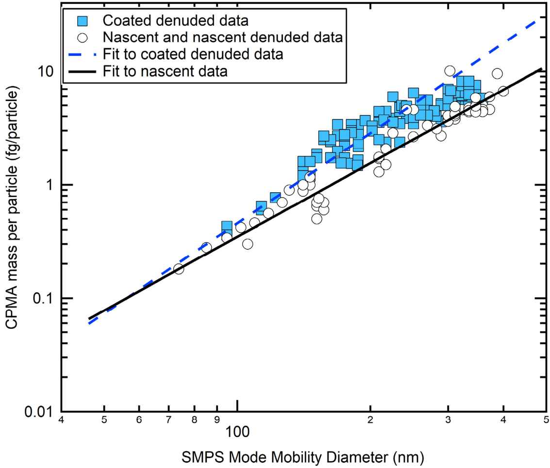
Figure S2. Observations and fits of CPMA mass per particle as a function of the SMPS mode number-weighted mobility diameter for methane diffusion flame soot particles. The blue squares show coated denuded observations and the dashed blue line is the power law fit to the coated-denuded data. The white circles are nascent observations and the black line is the power law fit to the nascent observations. Note that the fits to the coated-denuded data are for particles with mobility diameter < 260 nm since the large particles generally have thinner coatings and are therefore more fractal-like. The data were fit to a power law function (see eqn. 8 in the main text). For nascent soot, fit parameters C and D_{f,m} were 1.70 \times 10^{-5} and 2.12, respectively, and for coated-denuded soot, fit parameters C and D_{f,m} were 2.44 \times 10^{-6} and 2.64, respectively.
