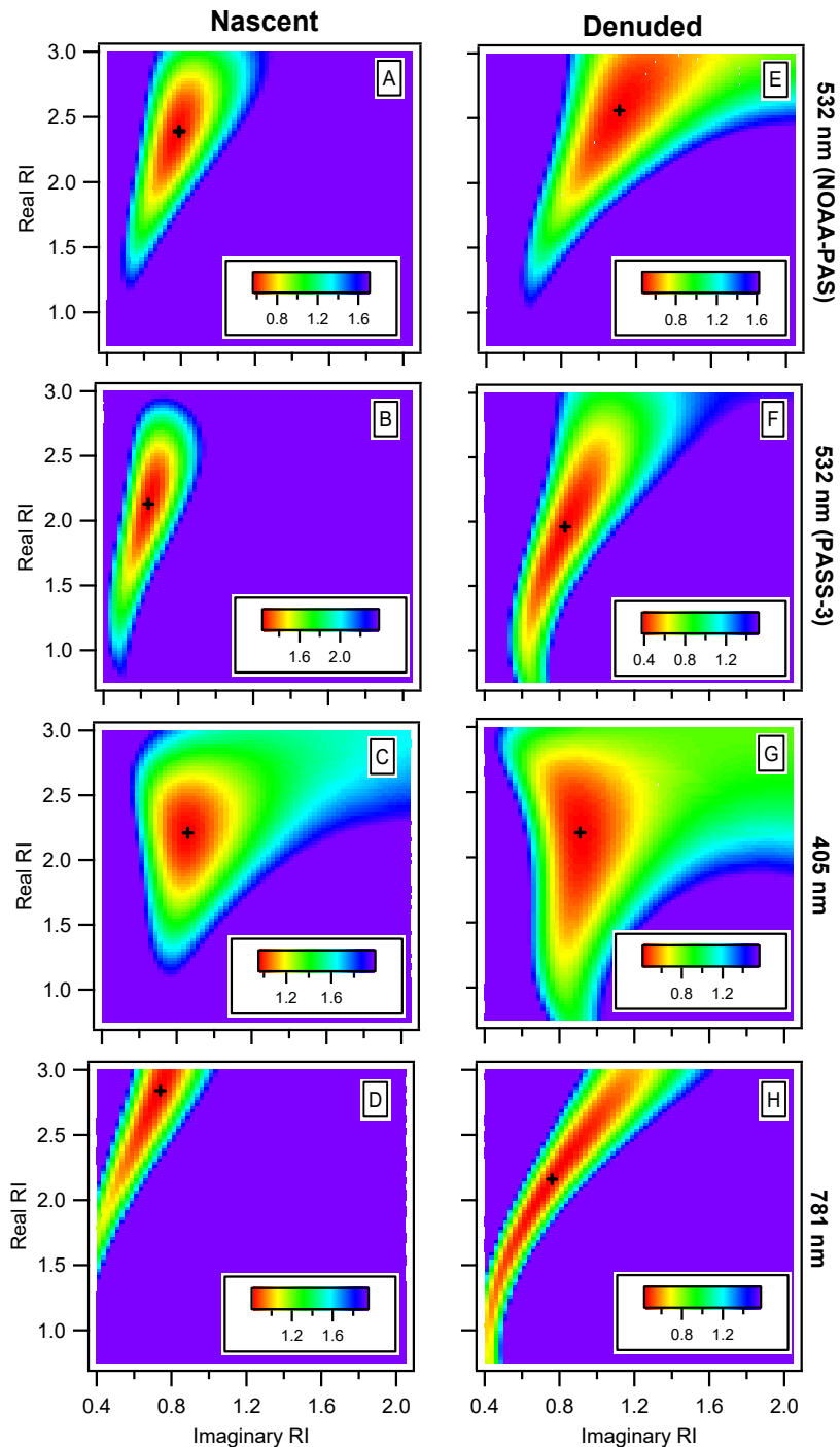
Figure S6. Image plots of the reduced \chi^2 values of Mie Theory fits to absorption for all ethylene flame (20 cm sampling height) data from BC2. Colors indicate reduced \chi^2 values, with the minima values shown as black crosses. Purple indicates the region beyond 1\sigma of the minimum reduced \chi^2 value ( \chi^2+1.11 ). Each panel is for a particular wavelength and soot type (nascent vs. thermodenuded). The left column (A-D) is for nascent soot. The right column (E-H) is for denuded soot. Panels A and E are \lambda = 532 nm NOAA PAS data, panels B and F are \lambda = 532 nm PASS-3 data, panels C and G are \lambda = 405 nm PASS-3 data, and D and H are \lambda = 781 nm PASS-3 data.
