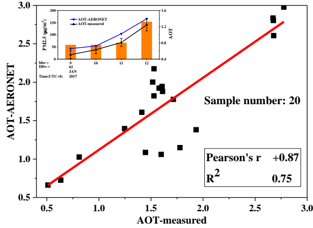
5 Figure 2: Correlation of the AOT values deduced from AERONET sites and ground-based LiDAR data. The inserted chart gives the changes of PM2.5 mass concentration and AOT values at the ground-based LiDAR site on January 2, 2017.
