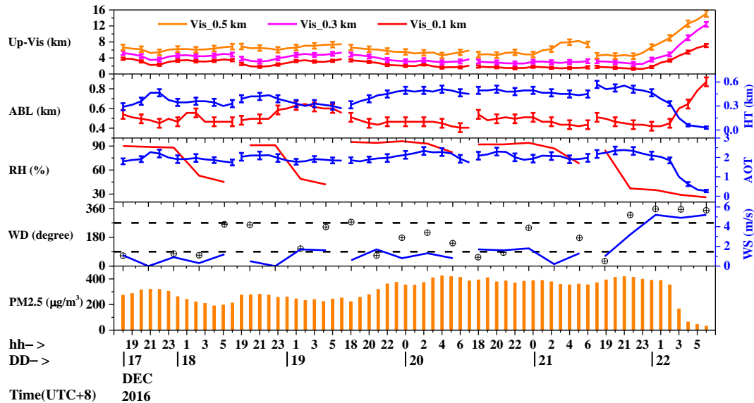
5 Figure 4: Hourly variation of multiplatform data between December 17, 2016 and December 22, 2016 in the northwest of downtown Beijing.
