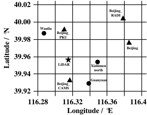
10 Figure 1: Geographic coordinate of ground-based LiDAR site (star), air quality monitoring sites (circle) and AERONET sites (upper triangle).
