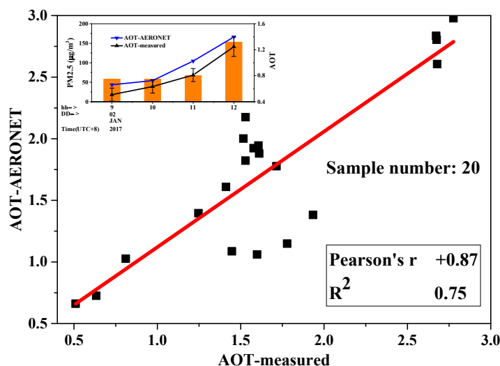
Figure R2: Correlation of the AOT values deduced from AERONET sites and ground-based LiDAR data. The inserted chart gives the changes of PM 2.5 mass concentration and AOT values at the ground-based LiDAR site on January 2, 2017.
