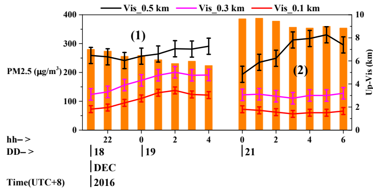
Figure R3: Hourly variation of Up-Vis and PM2.5 mass concentration in certain period.
