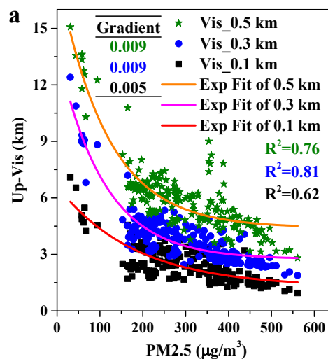
Figure R1: Scatter plot of PM 2.5 mass concentration and Up-Vis in the northwest of downtown Beijing. The inserted table denotes the statistical gradient of Up-Vis at different altitudes.
