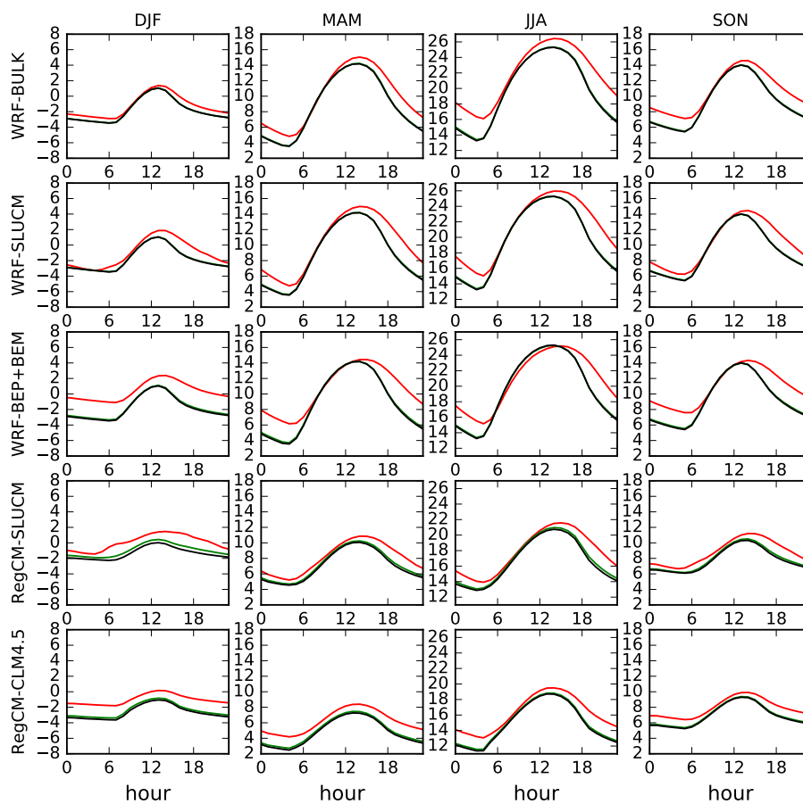
Figure 6. Averaged temperature daily cycles ( ^{\circ}\text{C} ) in the Prague city center (red), in its surroundings (green) and those simulated with the urban surface removed (black).
