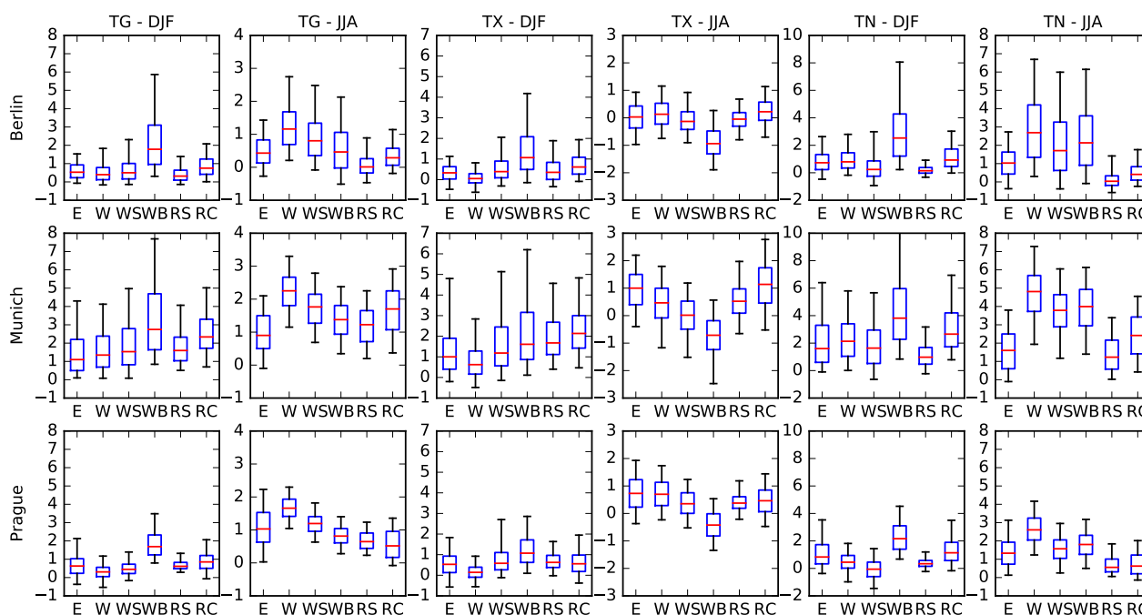
Figure 4. Distributions of temperature differences ( ^{\circ}\text{C} ) between city centres and their surroundings in winter and summer season given by station data (E), WRF-BULK (W), WRF-SLUCM (WS), WRF-BEP+BEM (WB), RegCM-SLUCM (RS) and RegCM-CLM4.5 (RC) model simulation. TG denotes temperature means, similarly TX and TN stand for maxima and minima, respectively. Whiskers indicate 5th and 95th percentile.
