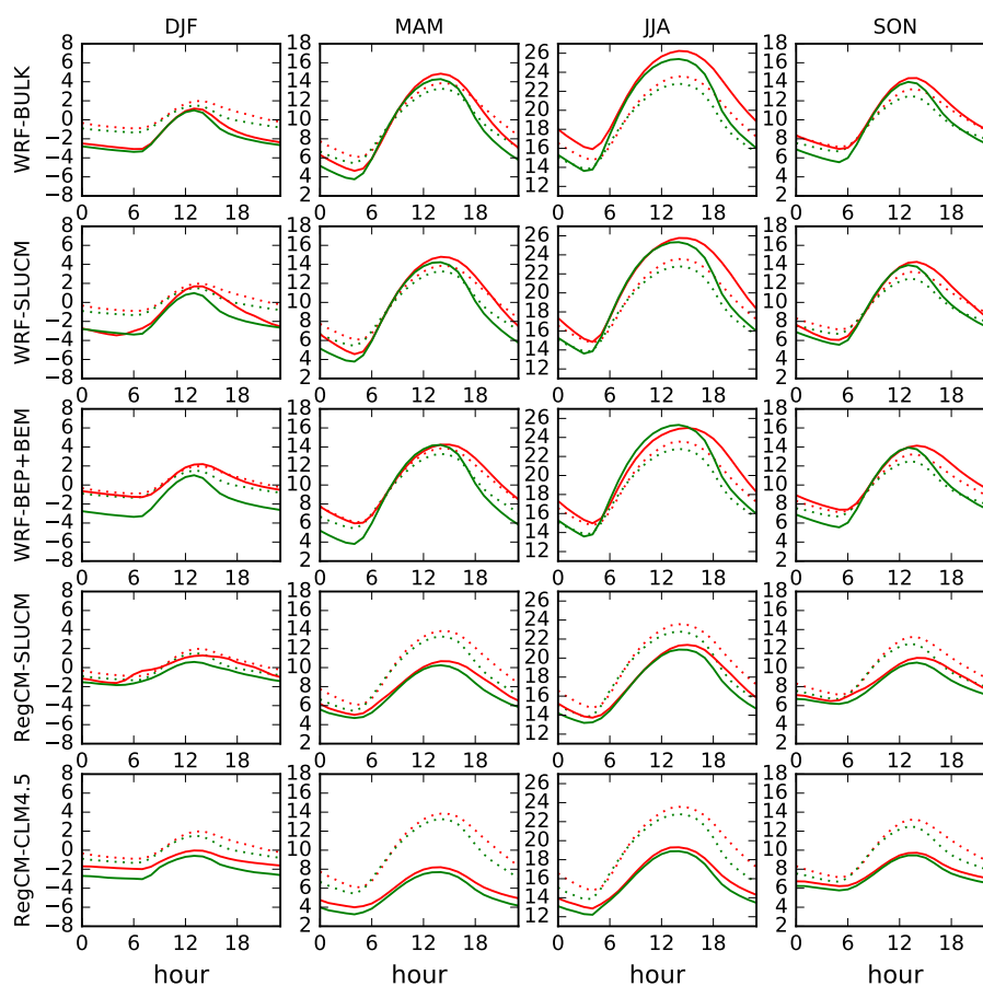
Temperature in Prague city center (red), vicinity (green), models (solid), ref. (dotted)
