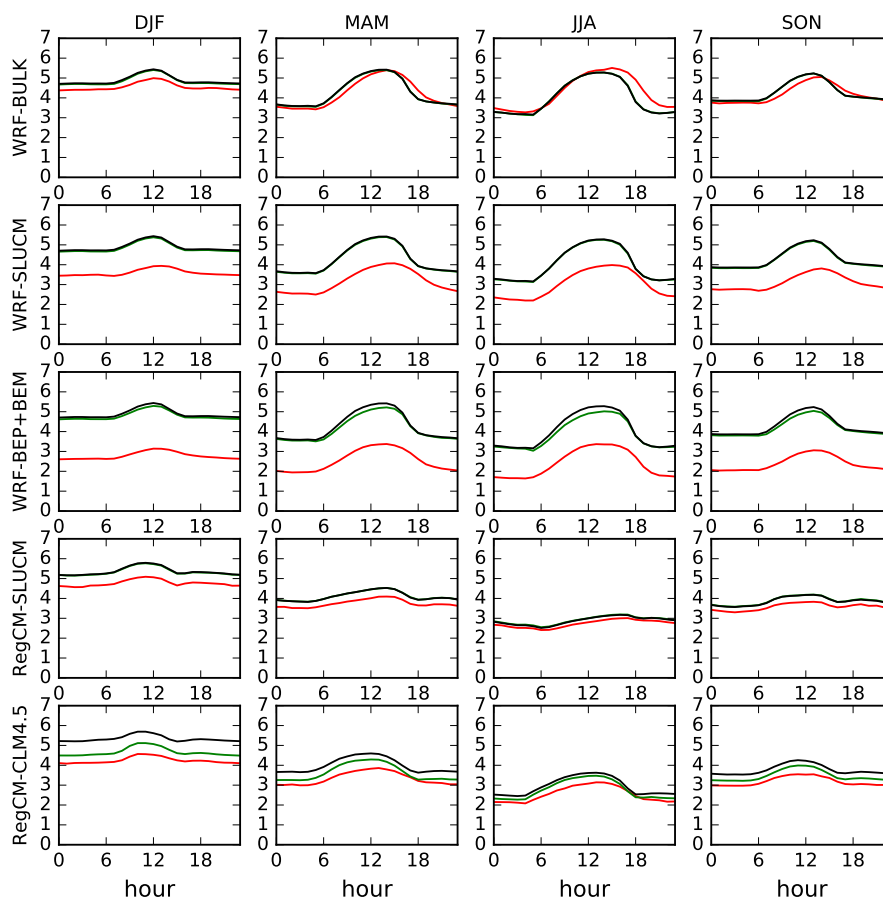
Figure 8. Averaged horizontal wind speed daily cycles ( \text{m s}^{-1} ) in the Prague city center (red), in its surroundings (green) and as simulated with the urban surface removed (black).
