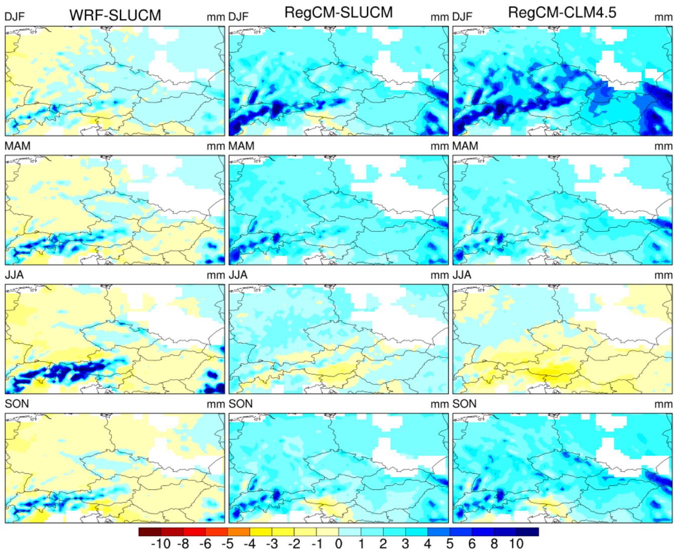
Figure 3. Spatial distribution of averaged daily precipitation biases (mm) for individual seasons and simulations. The white color indicates missing reference data.
