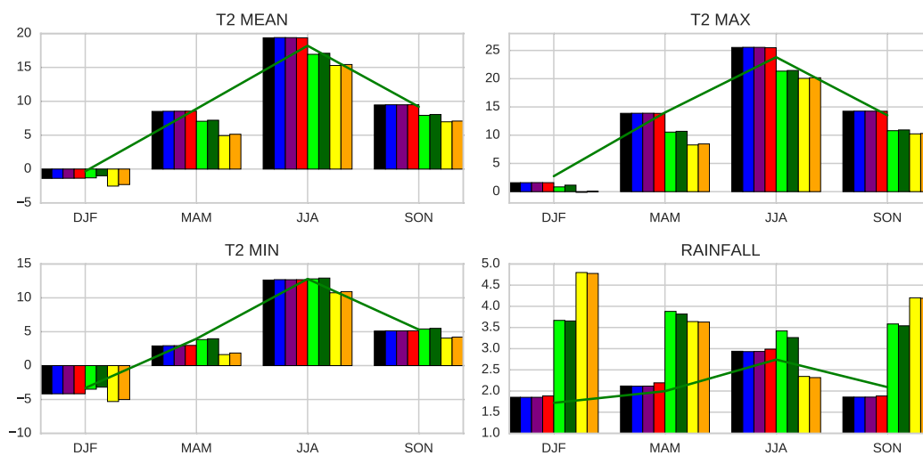
Figure 2. Averaged seasonal modelled temperatures (in °C) and precipitation (mm) for individual model simulations: Black – WRF–woU, blue – WRF–BULK, purple – WRF–SLUCM, red – WRF–BEP+BEM, light green – RegCM–SLUCM–woU, dark green – RegCM–SLUCM, yellow – RegCM–CLM4.5–woU, orange – RegCM–CLM4.5. Green curve stand for the seasonal values given by E-OBS.
