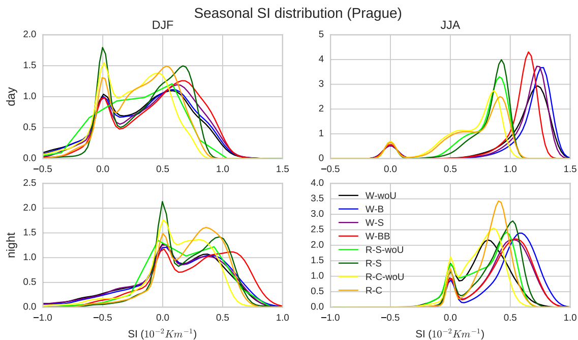
Figure 12. Seasonal distributions of the Stability Index (SI; in 10^{-2} \text{K m}^{-1} ) for the city of Prague, given by all simulations. The day represents the time between 11–16 UTC, the night represents the time between 23–04 UTC.
