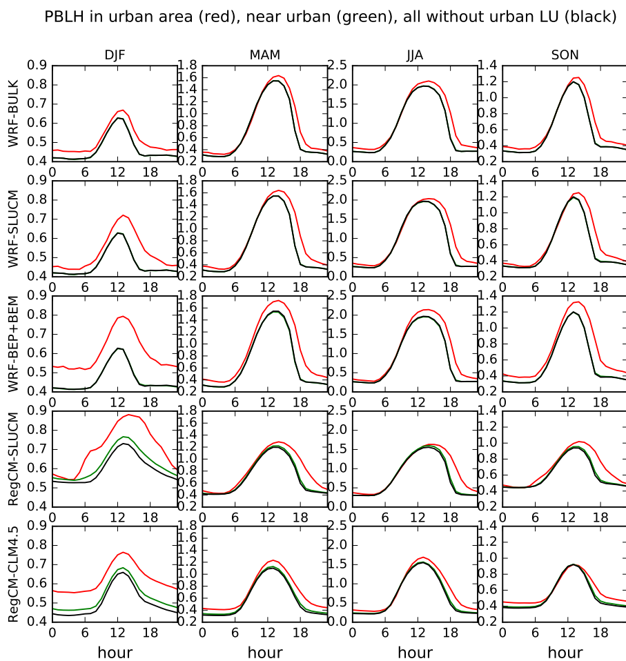
Figure 7. Averaged daily cycles of the planetary boundary layer height (PBLH) in the Prague city center (red), in its surroundings (green) and as simulated with the urban surface removed (black) in kilometres.
