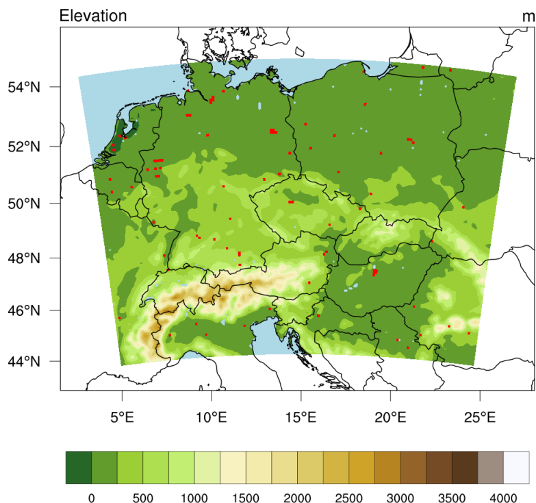
Figure 1. Position of the model domain with model topography in 10 km resolution (m). Grid-boxes with dominant urban land-use are marked by red color.
