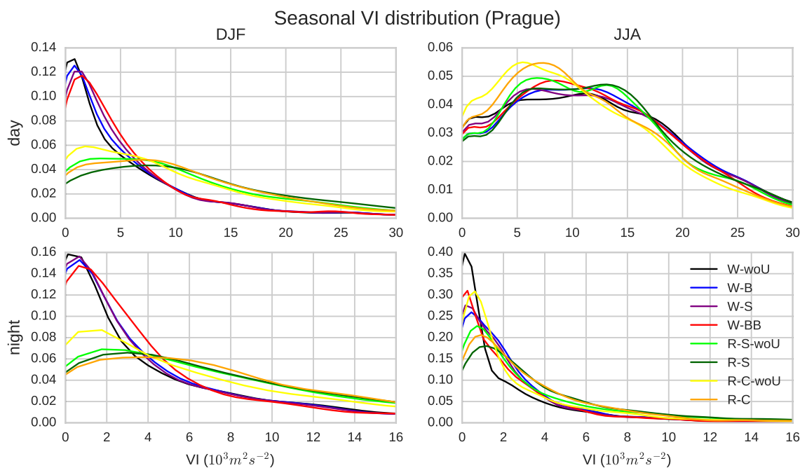
Figure 11. Seasonal distributions of the Ventilation Index (VI; in 10^3 \text{m}^2 \text{s}^{-2} ) for the city of Prague, given by all simulations. The day represents the time between 11–16 UTC, the night represents the time between 23–04 UTC.
