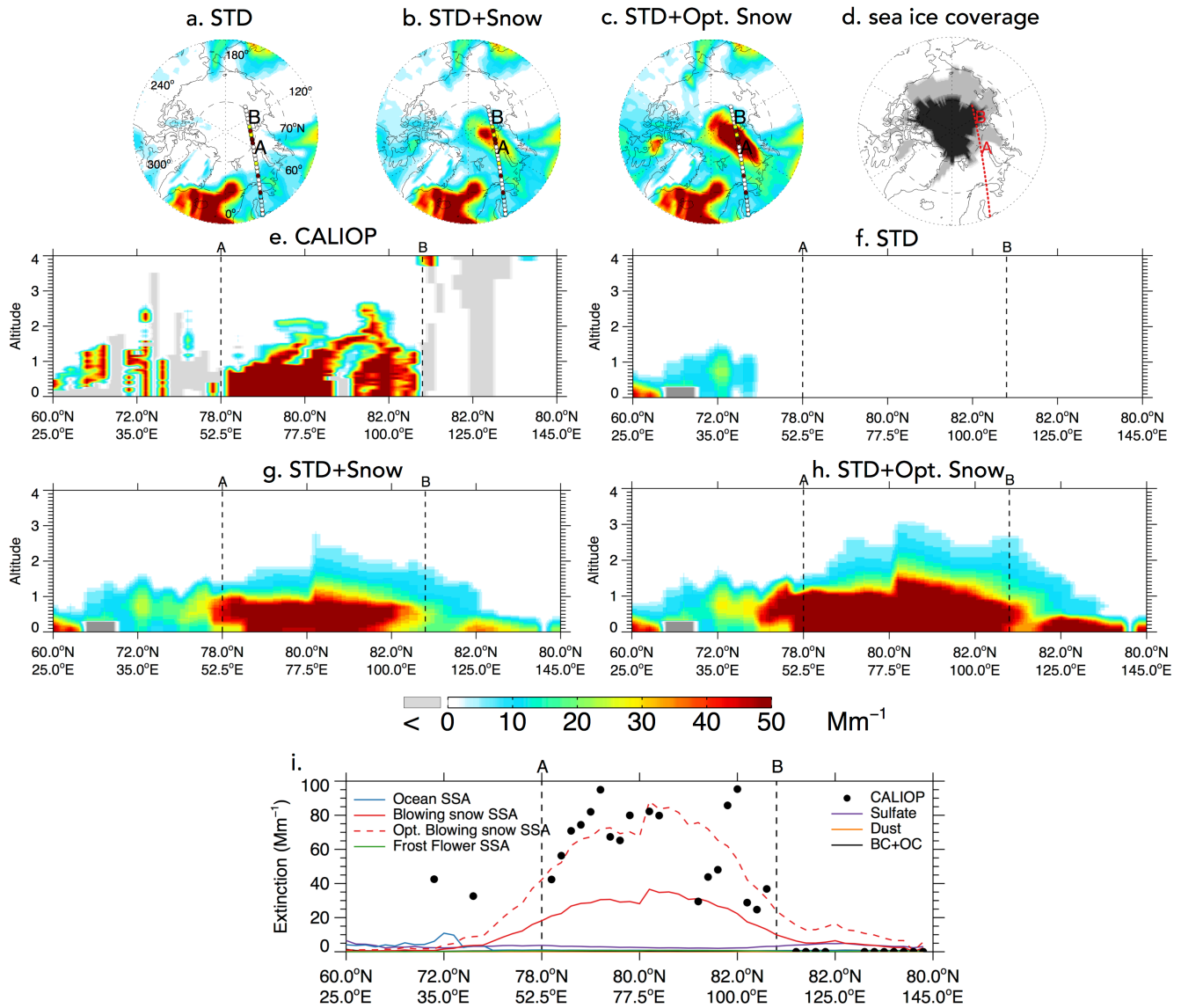
5 Figure 7. November 6, 2008 case study of a blowing snow SSA feature over the Arctic. Top panels: Spatial distribution of mean aerosol extinctions below 2 km altitude for the (a) STD, (b) STD+Snow, and (c) STD+Opt. Snow GEOS-Chem simulations. The CALIOP nighttime overpass at 00:58–01:12 UTC is displayed on the top panels, with filled circles color-coded according to observed mean extinction coefficients below 2 km. The overpass intercepts the SSA blowing snow feature between points A and B. Panel (d) shows the MERRA sea ice coverage on November 6, 2008, with light gray shading indicating FYI and black shading for MYI. Panels (e–h) show the observed and simulated vertical cross-sections of aerosol extinction coefficients along the CALIOP overpass. The light gray shading in (e) indicates that no valid data is available for CALIOP. The dark gray shading in (f–h) shows the local topography in the model. Panel (i) shows the 0–2 km CALIOP mean aerosol extinctions and the contributions of different aerosol types in the GEOS-Chem simulations: sulfate aerosol, dust, black carbon and organic carbon (BC+OC), open ocean SSA, blowing snow SSA, Optimized blowing snow SSA, Frost Flower SSA. 10
