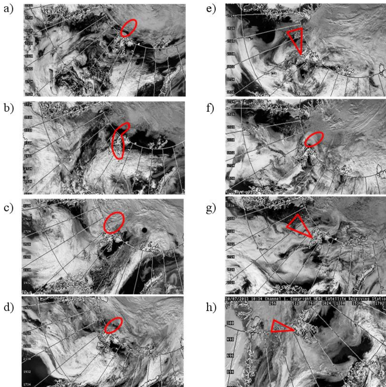
Figure S1: Satellite images for flights M191 – M198 from AVHRR Channel 1, visible. Red circles indicate approximate area of flight track.
