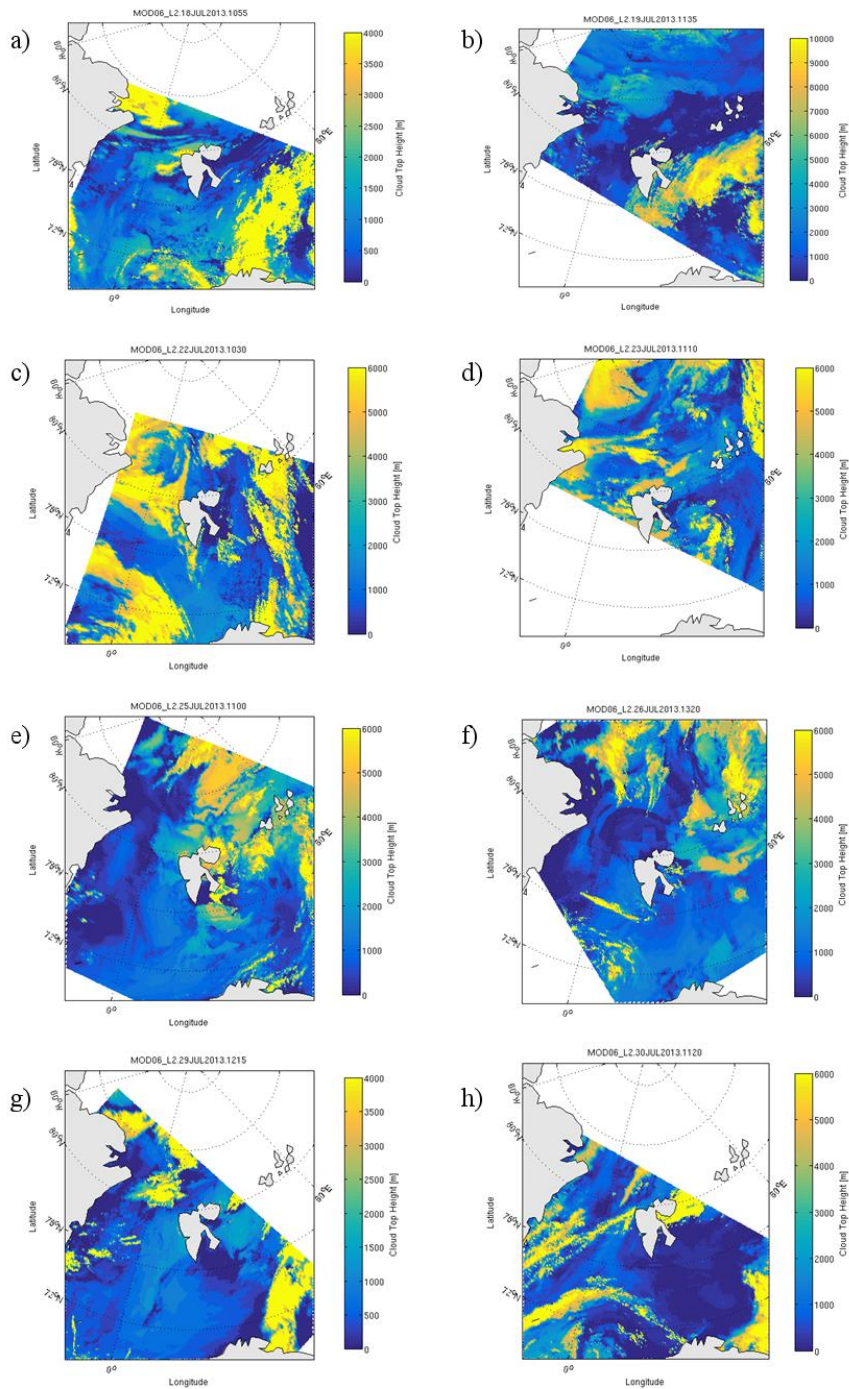
Figure S2: Cloud top height MODIS satellite retrievals shown for all flights. Note that the colorbar maximum value has been capped in all cases to allow structures to be seen clearly.
