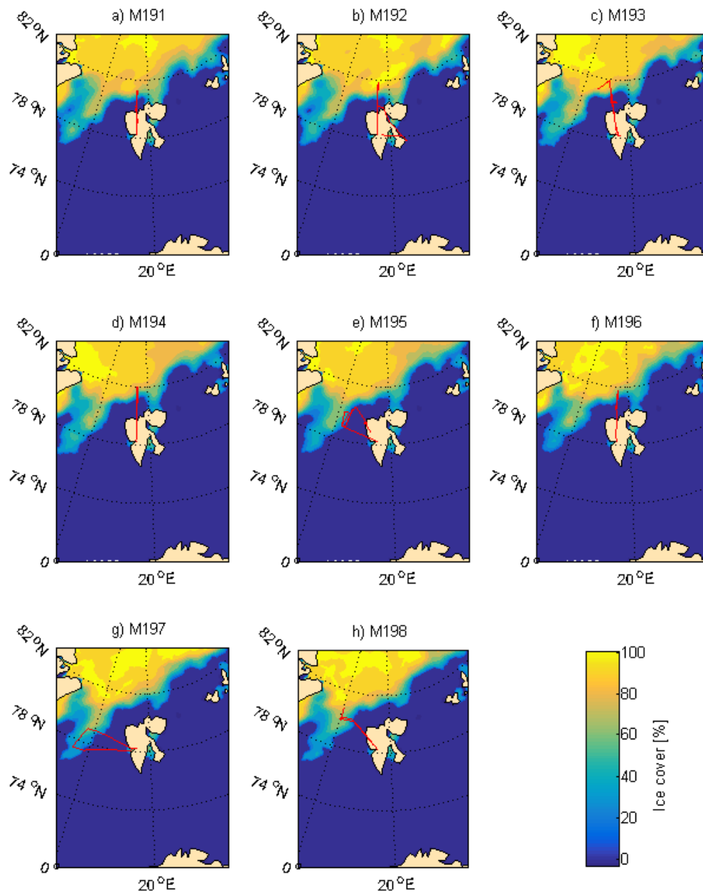
Figure S3: Flight track of MASIN aircraft for all 8 science flights. Also shown is the sea-ice cover (see colorbar) from NSIDC data.
