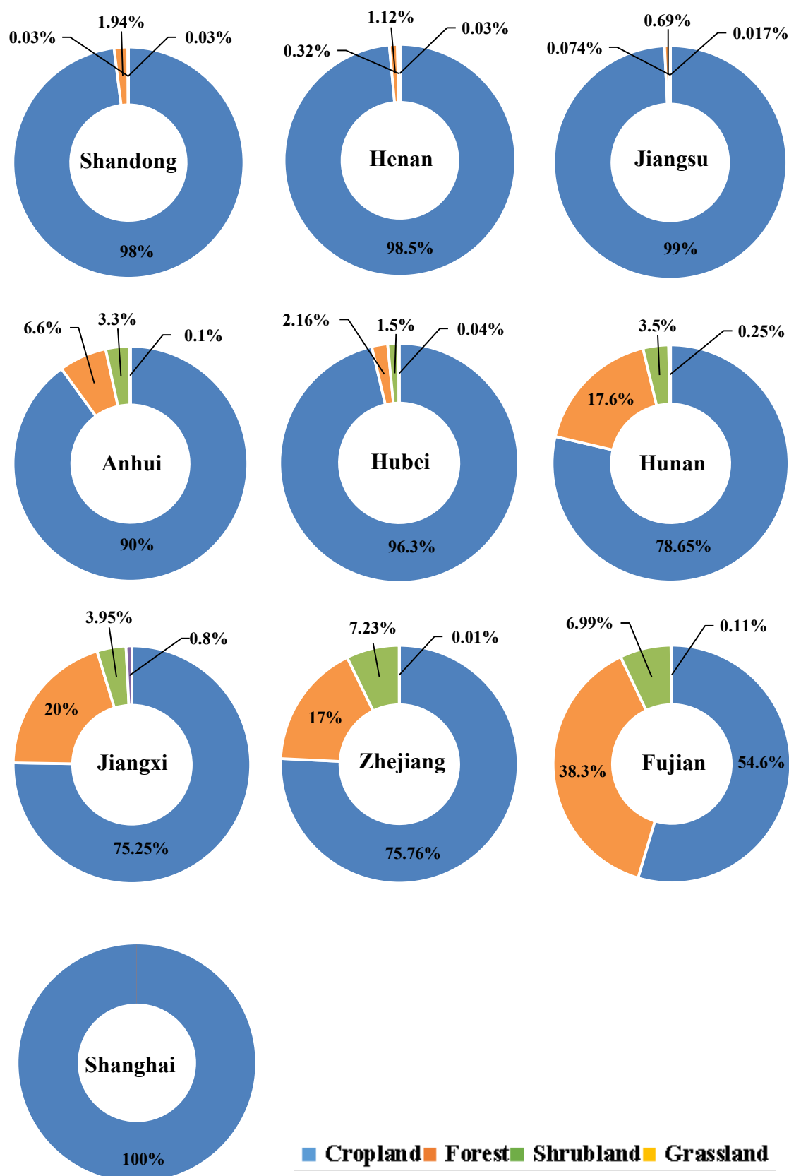
Figure 3. The averaged contributions of different biomass burning types to PM_{2.5} emission in each province.
