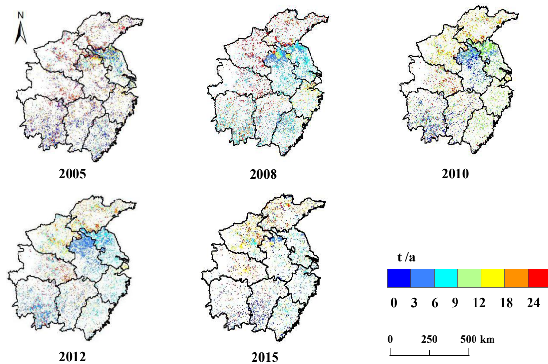
Figure 10. Annual spatial distribution ( 1 \text{ km} \times 1 \text{ km} ) of \text{PM}_{2.5} emission from opening biomass burning in Central and Eastern China.
