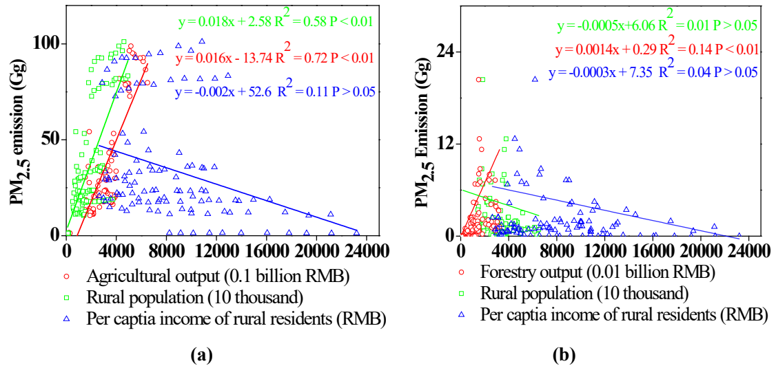
Figure 12. Correlation between PM_{2.5} emission from crop residue burning and agricultural output , rural population, per capita incomes of rural residents (a) and correlation between PM_{2.5} emission from forestry fire burning and forestry output, rural population, per capita incomes of rural residents (b) in different provinces from 2003 to 2015.
