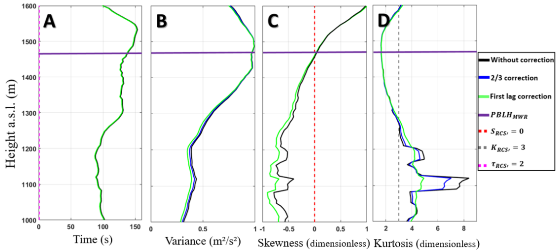
Figure 7 – A- Vertical profile of Integral time scale ( \tau_{RCS'} ). B - Vertical profile of variance ( \sigma_{RCS'}^2 ). C - Vertical profile of Skewness ( S_{RCS'} ). D - Vertical profile of Kurtosis ( K_{RCS'} ).
