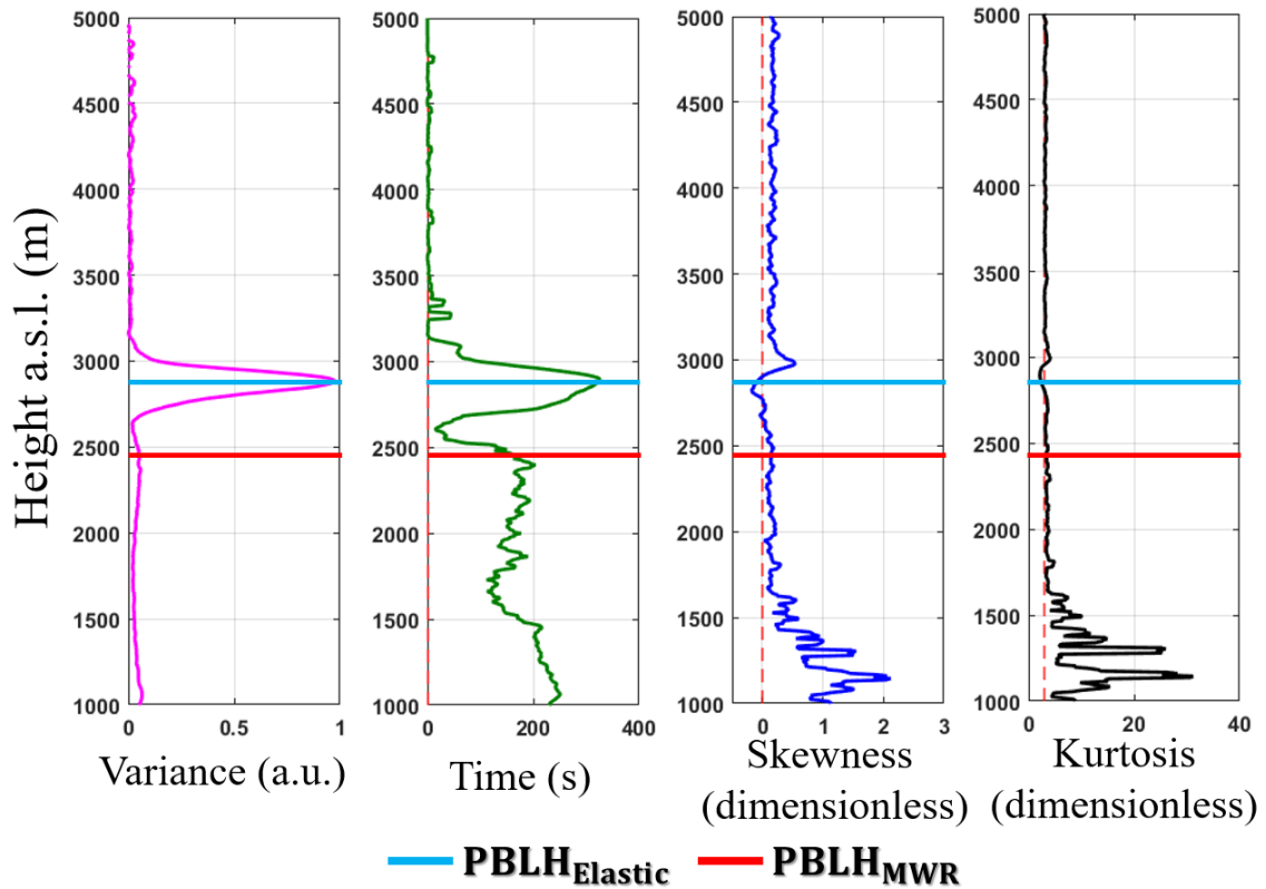
Supplementary Material - Figure 6 - Statistical moments obtained from elastic lidar data at 15 to 16 UTC - 19 May 2016. From left to right: variance [ \sigma_{RCS'}^2 ], integral time scale [ \tau_{RCS'} ], skewness [ S_{RCS'} ] and kurtosis [ K_{RCS'} ].
