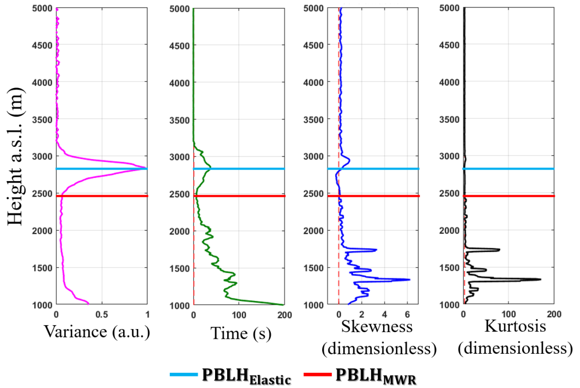
Supplementary Material - Figure 5 - Statistical moments obtained from elastic lidar data at 14 to 15 UTC - 19 May 2016. From left to right: variance [ \sigma_{RCS'}^2 ], integral time scale [ \tau_{RCS'} ], skewness [ S_{RCS'} ] and kurtosis [ K_{RCS'} ].
