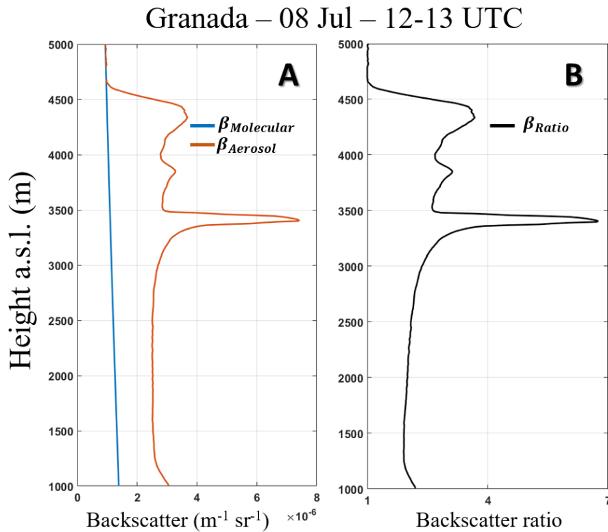
Figure 14 – (A) \beta_{\text{Molecular}} (blue line) and \beta_{\text{Aerosol}} (orange line). (B) \beta_{\text{Ratio}} (black line). All profiles were obtained from the 532 nm lidar signal
