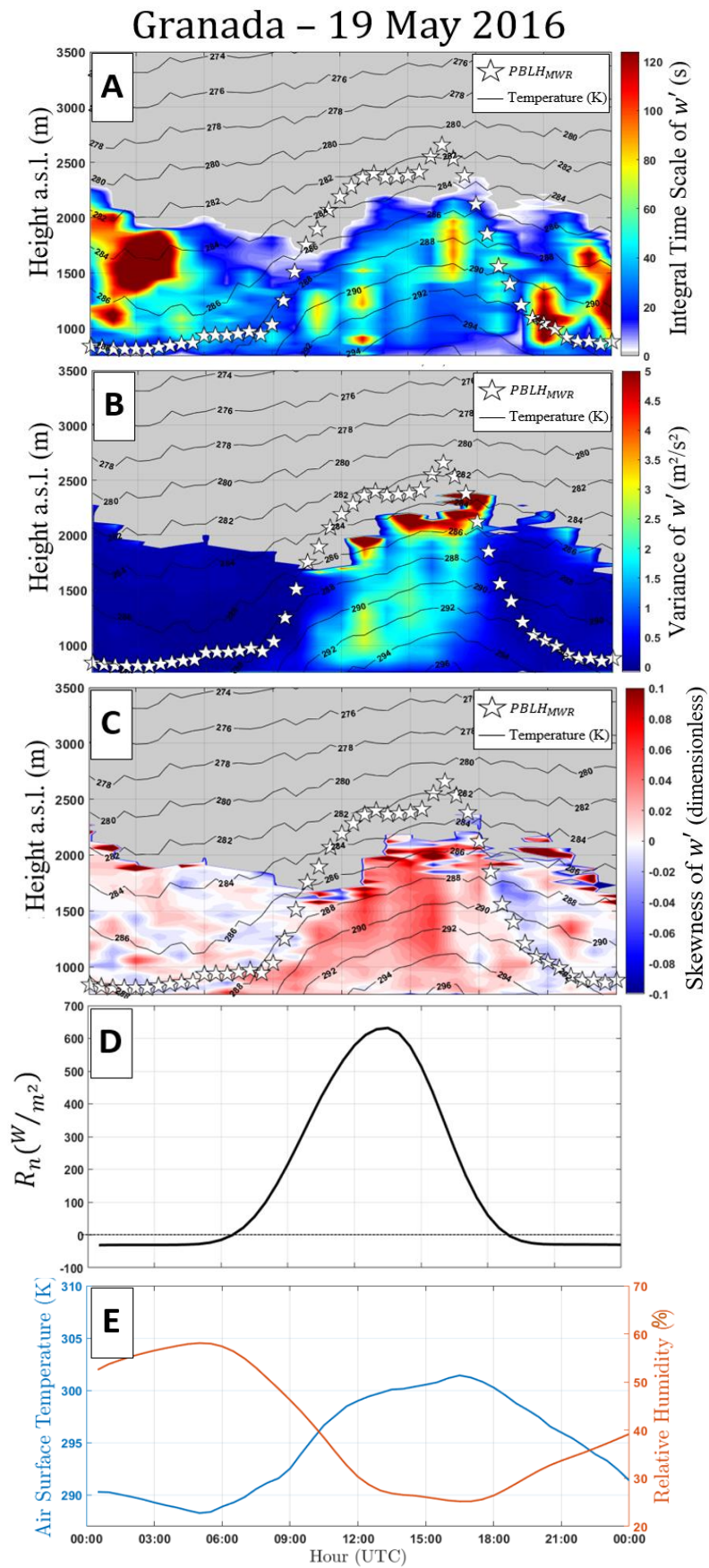
Figure 8 – A – integral time scale [\tau_{wv}] , B – variance [\sigma_{wv}^2] , C – skewness [S_{wv}] , D – net radiation [R_n] , E – Air surface temperature [blue line] and surface relative humidity [RH] – orange line]. In A, B and C black lines and white stars represent air temperature and PBLH_{MWR} , respectively.
