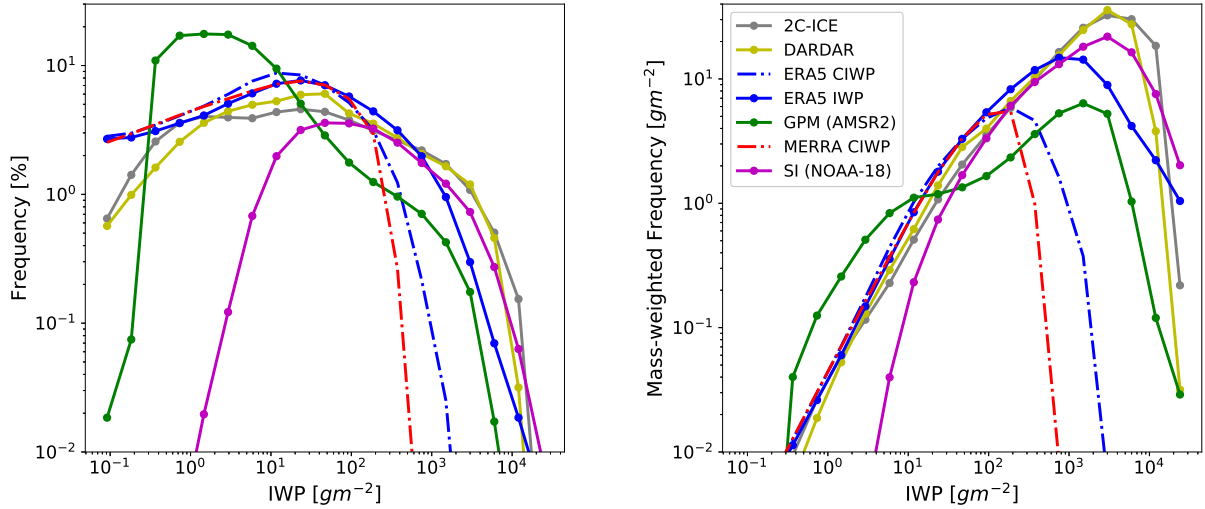
Figure 2. Probability distribution function of IWP values from native resolution level 2 data and 0.5^\circ reanalysis data. This is shown as a percentage (left) and weighted by mass (right), i.e. summing values in the right panel yields approximately the near-global mean. These data include daytime values spanning 60^\circ\text{N} - 60^\circ\text{S} from 2015, with 2C-ICE (2008) and SI (2013) the exceptions due to availability. DARDAR data were treated with a running mean of six pixels to approximate a passive microwave footprint. The frequencies shown account for zero values, which given in the text.
