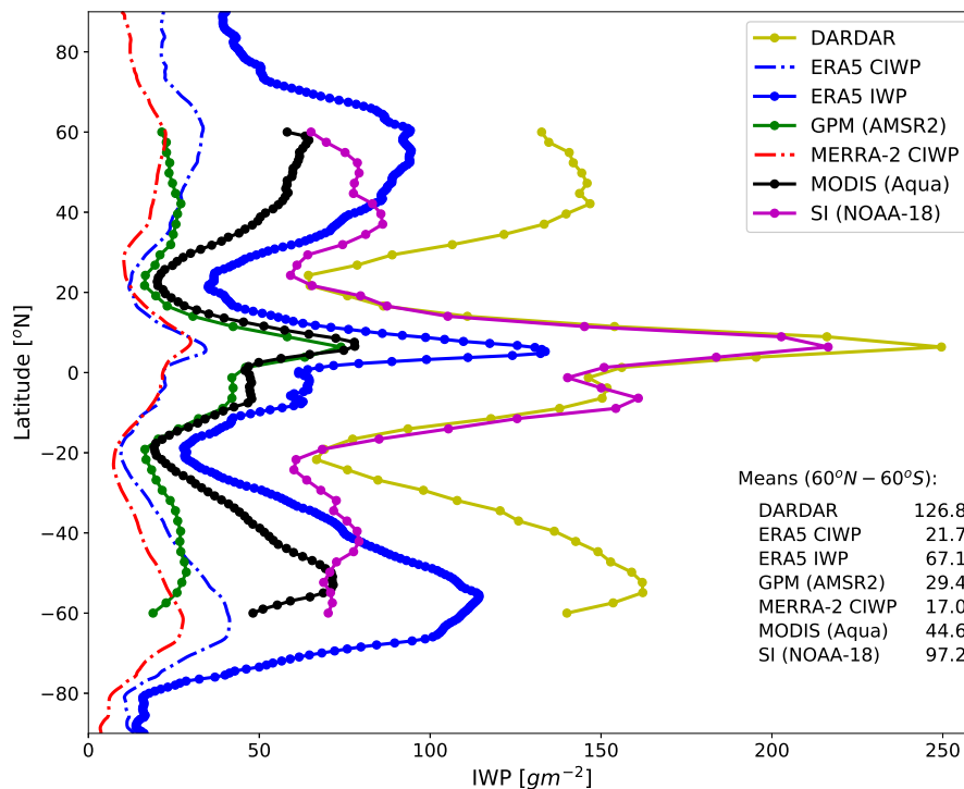
Figure 3. Zonal means of IWP, centred on A-Train daytime observations. 2015 is used for all datasets excepting SI (2013). ERA5 zonal means are presented for both non-precipitating cloud ice (CIWP) and total ice (CIWP+SIWP=IWP) for better comparison with MERRA-2 and the observations, respectively. The observational datasets are cut off at 60^\circ latitude to mitigate relative sampling biases, with near-global mean values displayed.
