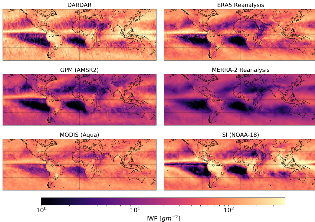
Figure 1. Global mean IWP maps from six datasets: 4 satellite datasets (DARDAR, GPM, MODIS, SI) and 2 reanalyses (ERA5, MERRA-2). 2015 data are used for all datasets except SI (2013) and DARDAR (2008-2015) due to data availability and desire for greater sampling, respectively. Daytime data were used exclusively to improve comparability with MODIS and the extended CloudSat record. Note that MERRA-2 constitutes non-precipitating ice only, whereas the other panels represent total ice.
