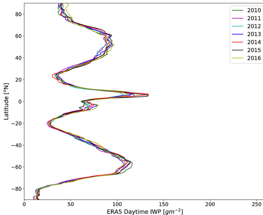
Fig. 1. 2010 to 2016 ERA5 zonal mean IWP
