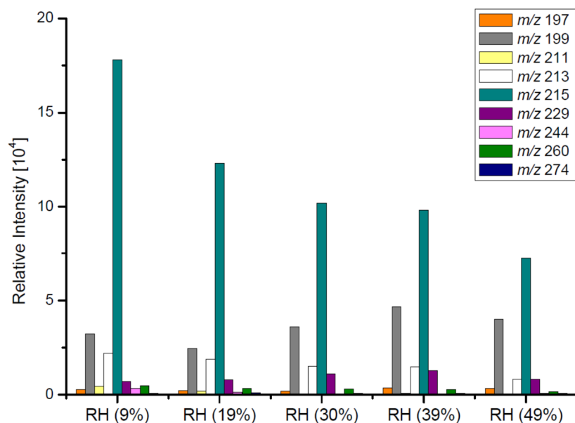
Figure 3. LC-MS chromatographic responses of OSs and NOSs from the non-acidic seed experiments (non-acidic).
