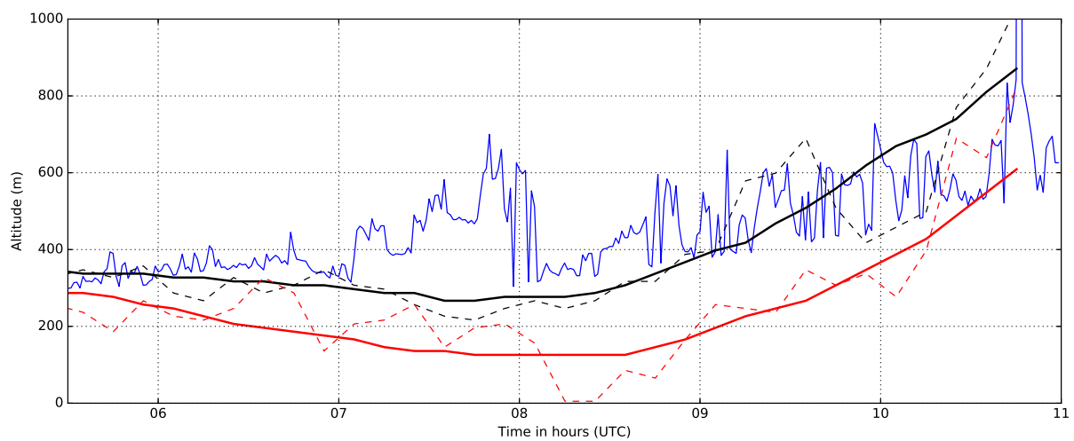
Figure 14. As Fig 5b but with results from CASIM_200 shown in red.
