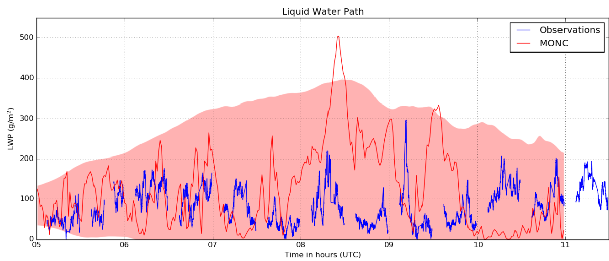
Figure 13. As Fig 8 but for CASIM_200.
