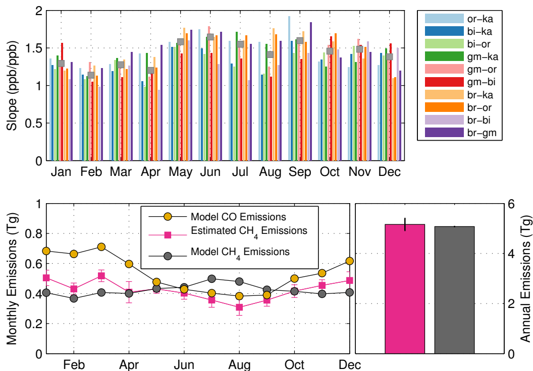
Figure 5. This figure shows the results from the modeling experiment using GEOS-Chem. The top panel shows the model \Delta X_{CH_4} - \Delta X_{CO} slopes for each month and pair of stations (indicated by the colours). The median slopes for each month are overlaid in grey squares. The bottom left panel shows the model carbon monoxide emissions (excluding VOC and methane oxidation) and the model methane emissions. The inferred methane emissions from our tracer-tracer slope method are plotted in pink squares. The bottom right panel shows the annual methane emissions from the tracer-tracer slope method and the model.
