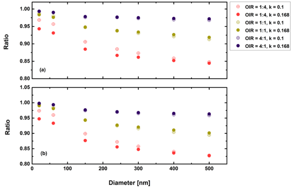
Figure 11: Ratio of radiative forcing of LLPS to homogenous case under 70 % RH (a) and dry condition (0 % RH). (b) both for AAE = 2 and albedo a = 1 .
