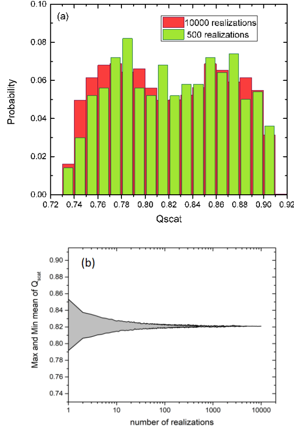
Figure 2 (a): Probability distribution of Q_{\text{scat}} for a phase separated particle with the eccentric core positioned at 500 random locations (green columns) and 10000 random locations (red column) within the volume of a 100 nm diameter particle at OIR = 1:4 n(\text{core}) = 1.429 + i \cdot 0 , n(\text{shell}) = 1.571 + i \cdot 0.84 . (b): Maximum and minimum of the mean for Q_{\text{scat}} for random realization of the position with the number of realizations used for the calculation.
