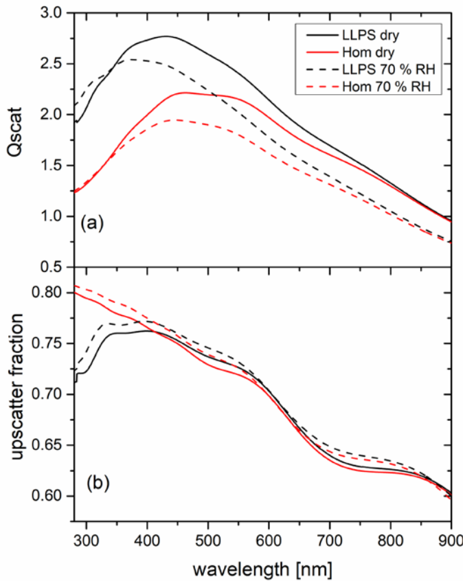
Figure 8 Shown are calculations for the limiting low albedo case. OIR 1:4, diameter 200 nm, k = 0.168 at 355 nm. (a): Scattering efficiency for the homogeneous morphology (red) and LLPS morphology (black) under dry and wet conditions (solid and dashed line, respectively) for particles of identical diameter (200 nm) and AAE = 2. (b): Up-scatter fraction for the homogeneous particle (red) and LLPS particle (black) under dry and wet conditions (solid and dashed line, respectively).
