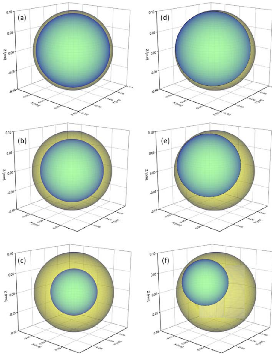
Figure 1: Schematic of a phase separated particle with a 100 nm radius to illustrate the thickness of the organic shell at (a): OIR = 1:4, (b): OIR = 1:1, and (c) OIR = 4:1 for concentric core-shell morphologies. (d) - (f) same for a single realization of an eccentric core-shell morphology. The calculations in this work use typically 500 such realizations, randomly oriented (with different distances of the inclusion from the center of the particles and different azimuth and polar angles) .The direction of incoming light is along the z-axis.
