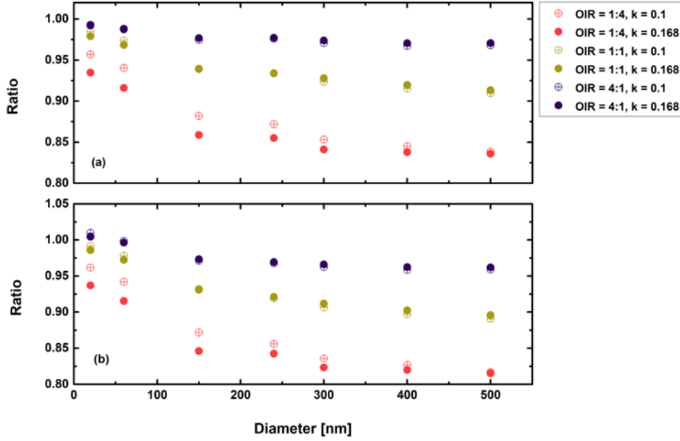
Figure 12: Ratio of radiative forcing of LLPS to homogenous case under 70 % RH (a) and dry condition (b) for AAE = 6 and albedo \alpha = 1 .
