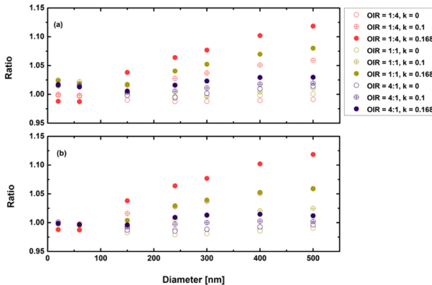
Figure 9: Ratio of radiative forcing of LLPS to homogenous case under 70 % RH (a) and dry condition (0 % RH). (b) both for AAE = 2 and albedo a = 0 .
