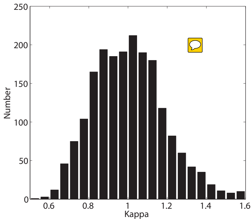
Figure 12. Histogram showing the 2171 \kappa values of all three seasons.
