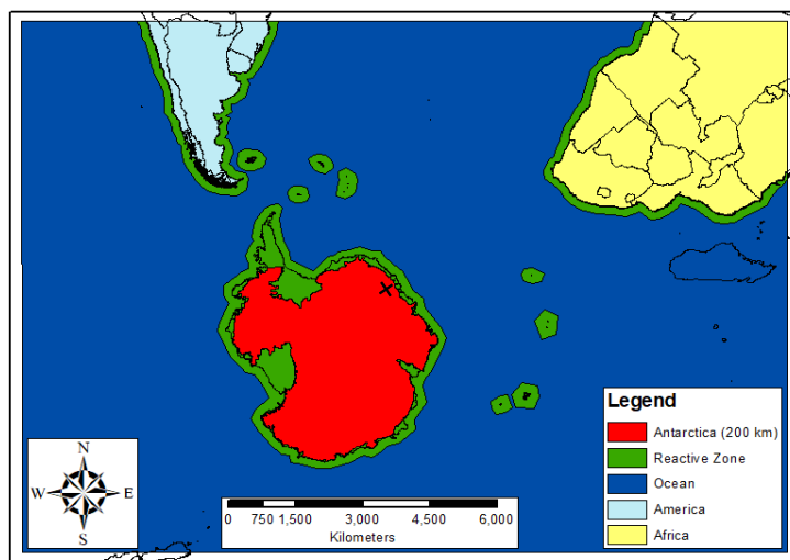
Figure 4. 5 different regions (Southern Ocean, Antarctic inland plateau, South America, Africa and Reactive Zone) that are used to track the percentage residence time in each region before arriving at PE from the NAME footprints.
