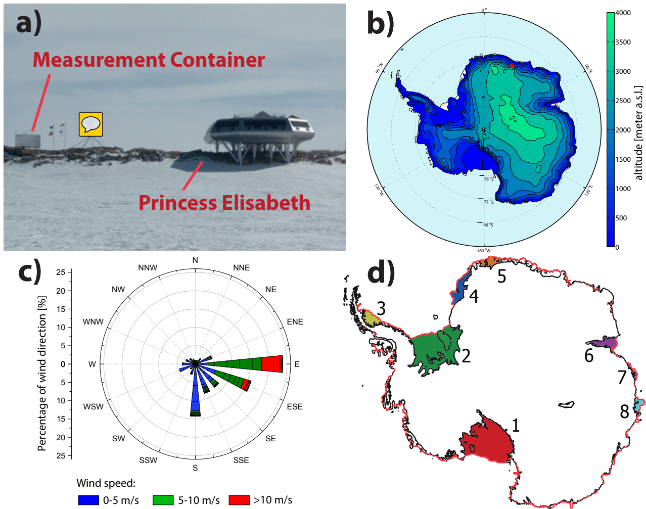
Figure 1. a) Picture of the Princess Elisabeth research station and the measurement container, where the aerosol measurements were performed, both located on the Utsteinen Nunatak ridge (view from ESE). b) Topographic map of Antarctica, the red dot shows the location of PE. This map was done using the Matlab mapping package M_Map. c) Wind direction and wind speed depicted as a wind rose for the third measurement period (December 18, 2015 to February 20, 2016). d) Map showing the location of the largest shelf ice regions in Antarctica: 1) Ross 2) Ronne-Filchner 3) Larsen C 4) Riiser-Larsen 5) Fimbul 6) Amery 7) West and 8) Shackleton shelf ice. The black line represents the coast line and the red line represents the ice edge. This map was created using Matlab and Antarctic Mapping Tools (Schaffer et al., 2016; Greene et al., 2017).
