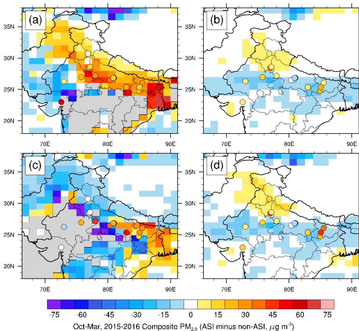
Figure 7. Composite of anomalies of PM 2.5 relative to monthly mean on days when ASI components (a) 10-m wind speed, (b) 500 mb wind speed, (c) precipitation, and (d) total ASI are met minus days when they are not during the period 1 October 2015 – 31 March 2016.
