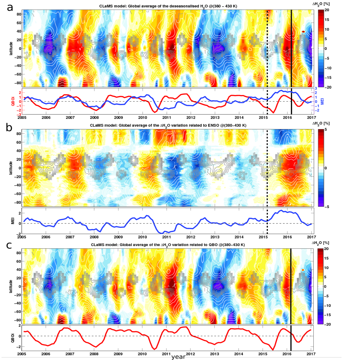
Figure 6. Latitude-time evolution of the global deseasonalised CLaMS H 2 O (a) together with the ENSO (b) and QBO (c) impact on lower stratospheric H 2 O in percent change from long-term zonal monthly means derived from the multiple regression fit and averaged between 380–430 K for the 2005–2016 period. Note that there is a factor of 4 difference in the color scales in Figs. 4b and 4c reflecting the difference in the magnitude of the H 2 O changes related to ENSO compared to those related to the QBO. Vertical black dashed line indicates February 2015 for the warm ENSO onset. Vertical black line indicates February 2016 for the QBO shift onset. Monthly averaged zonal mean zonal wind component, u (m·s -1 ), from ERA-Interim between 380–500 K is overplotted as solid white (westerly) and solid grey (easterly) lines.
