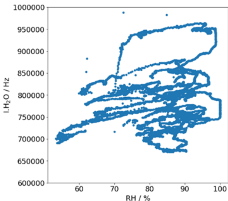
Fig 3. \text{I.H}_2\text{O} vs RH. No correlation is observed
