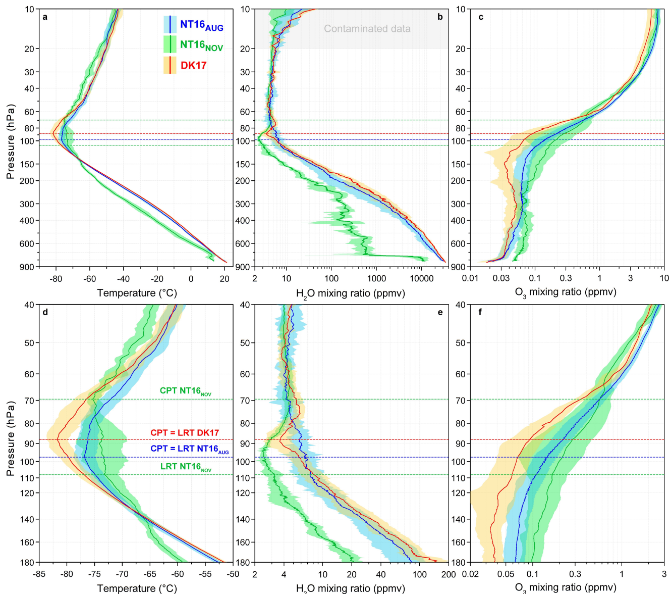
Figure 1. Mean profiles (solid lines) and standard deviations (color shading) of all measurements of temperature from RS41 (panels a, d), H 2 O mixing ratio from CFH (b, e) and O 3 mixing ratio from ECC (c, f) as a function of pressure, for NT16 AUG (blue), NT16 NOV (green) and DK17 (red). Dashed lines indicate the pressure levels of the average cold-point tropopause (CPT) and lapse-rate tropopause (LRT) for the different datasets. Upper row (a-c): measured profiles from the surface to 10 hPa. Bottom row (d-f): zoom into the tropopause region (40-180 hPa). The grey shaded area in panel b indicates the region of contaminated CFH data (see Section 3).
