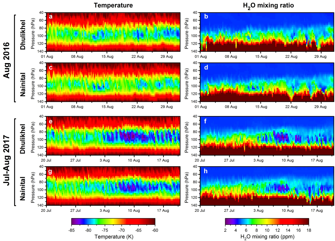
Figure 3. Time series of temperature (left column) and water vapor mixing ratio (right) as a function of pressure, from ECMWF operational analysis data (6-hourly, same horizontal and vertical resolution as given in caption of Figure 2) for the locations of NT (Panels c, d, g, h) and DK (a, b, e, f) during 1-31 August 2016 (a-d) and 20 July-21 August 2017 (e-h).
