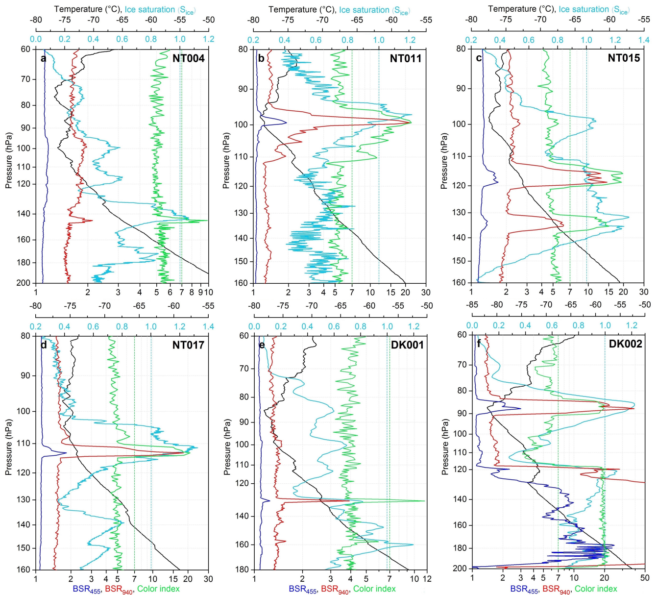
Figure 10. Examples of thin cirrus clouds measured during four individual soundings of the NT16 AUG campaign (panels a-d) and two soundings of the DK17 campaign (e-f). Solid lines show temperature (black), ice saturation (light blue), BSR at 455 nm ( BSR_{455} , blue), BSR at 940 nm ( BSR_{940} , red) and Color index (green). Vertical dashed lines mark the S_{ice} = 1 (light blue) and Color index = 7 (green) thresholds, used for cloud-filtering (see Section 6.1). Sounding identification numbers are noted in black at the top-right corner of each panel: for date, time and payload of each sounding, see Table S1 in supplementary material.
